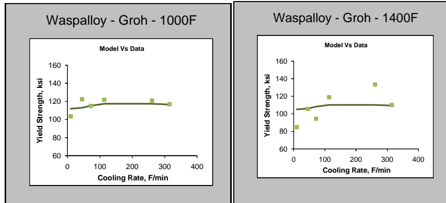
(a) (b) Figure 1. Predictions for Cooling Rate Effects (a) 1000 °F and (b) 1400 °F
