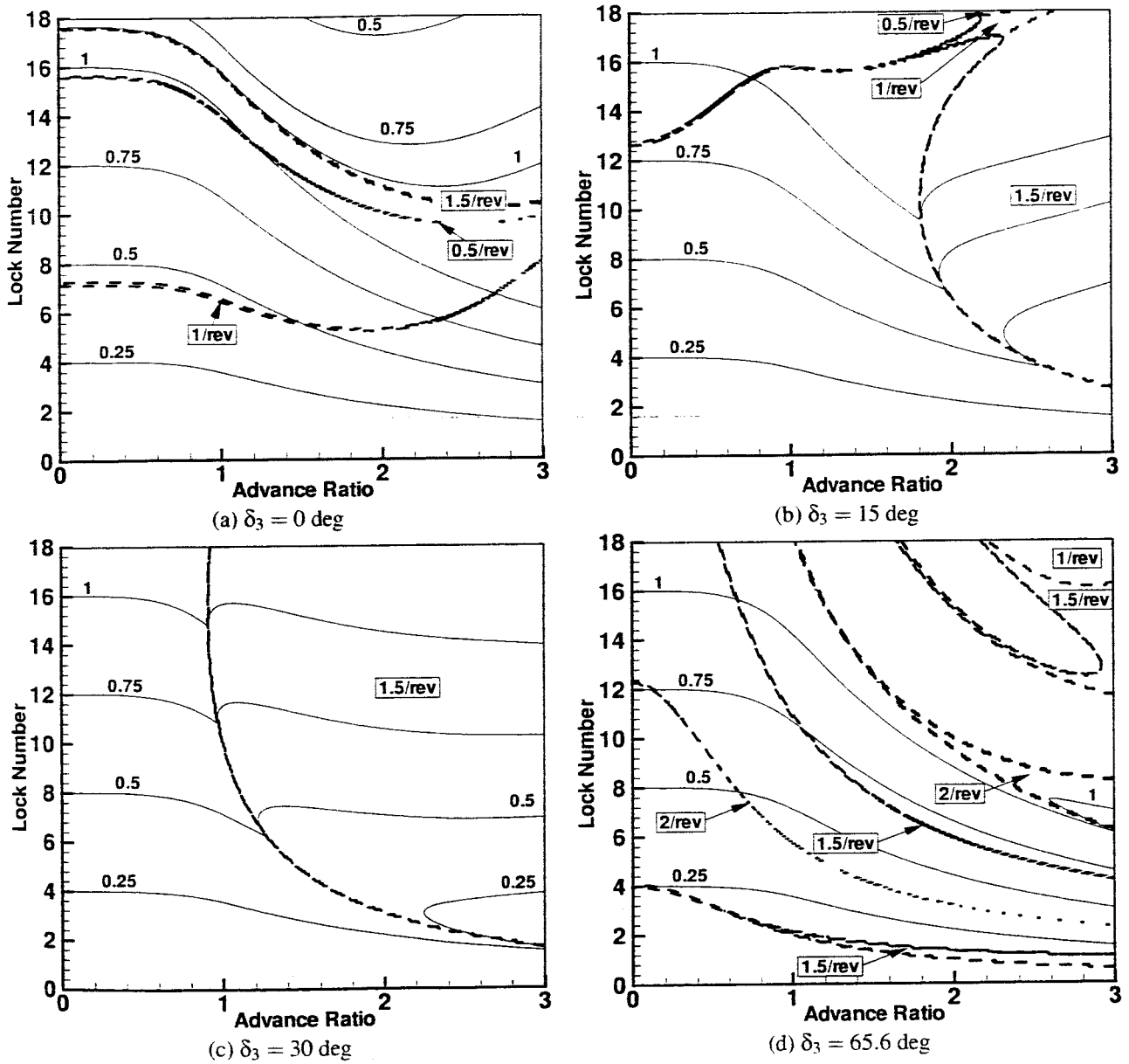
Fig. 4. Stability maps of only the coning mode of a rigid blade gimbaled rotor with coning hinge at 0.062R and 0, 15, 30, and 65.6 deg of \delta_3 , v_B = 1.1 .
