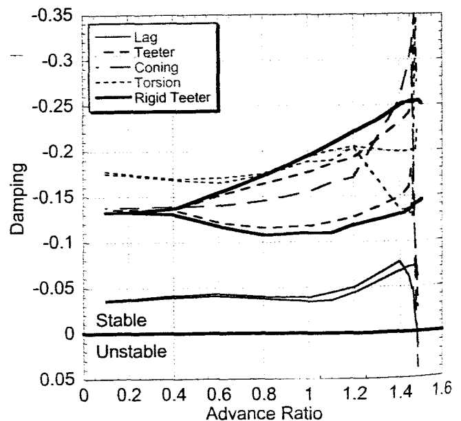
Fig. 31. Stability of elastic teetering rotor at tip speed V_T = 230 ft/sec and torsion frequencies of 4.5/rev.
