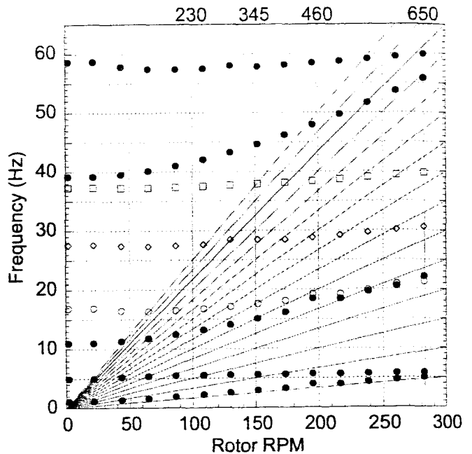
Fig. 30. Frequencies of the CAMRAD II elastic blade models with 4.5–6.5/rev torsion frequencies.
