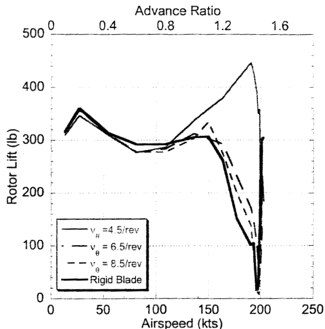
Fig. 34. Comparison of rotor lift for elastic and rigid blade teetering rotors, V_T = 230 ft/sec and elastic torsion frequencies of 6.5–8.5/rev and rigid.
