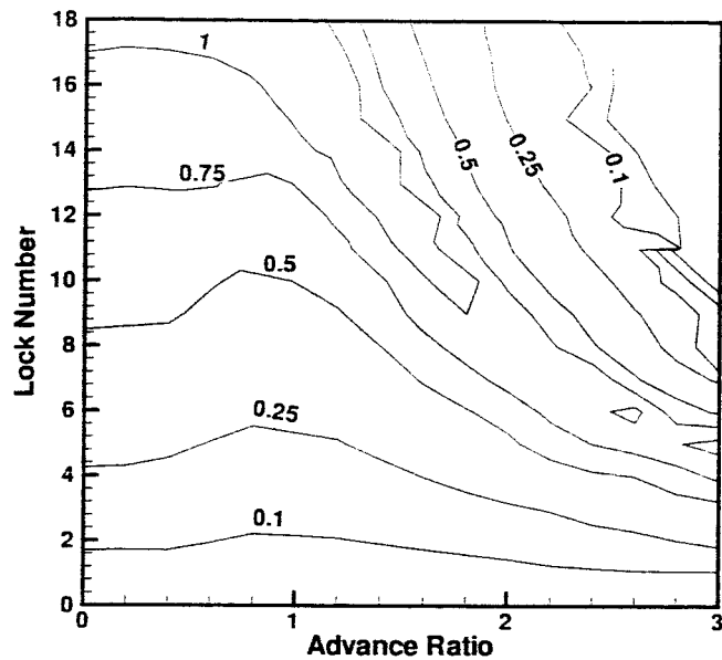
Fig. 8. Stability map for CarterCopter rotor from CAM-RAD II rigid blade model, \delta_3 = 10 deg, v_\beta = 1.0 , no trim.
