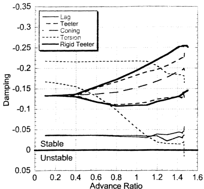
Fig. 32. Stability of elastic teetering rotor at tip speed V_T = 230 ft/sec and torsion frequencies of 6.5/rev.
