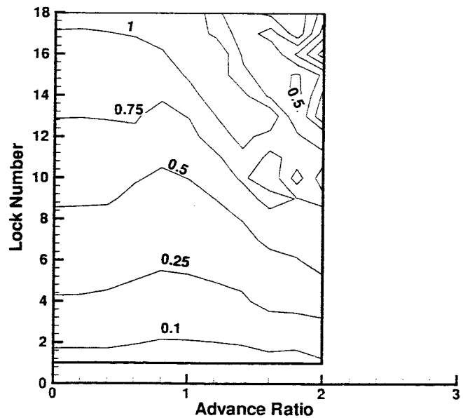
Fig. 9. Stability map for CarterCopter rotor from CAM-RAD II rigid blade model, \delta_3 = 10 deg, v_\beta = 1.0 , trimmed to autogyro condition.
