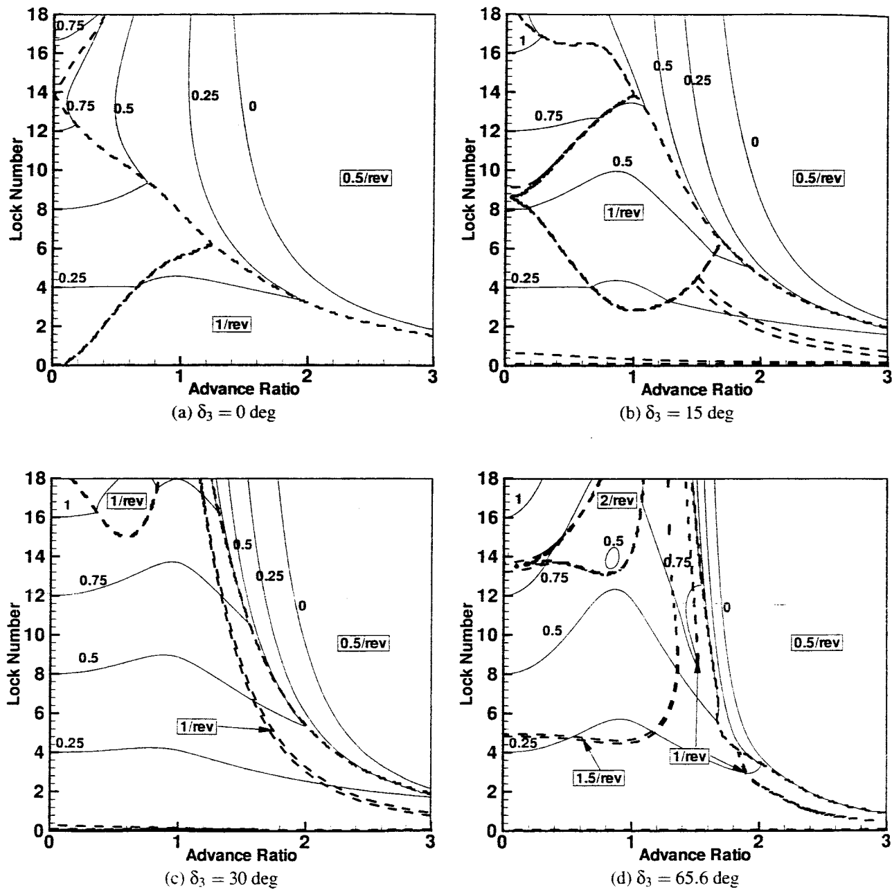
Fig. 3. Stability maps of cyclic modes of a rigid blade gimballed rotor at 0, 15, 30, and 65.6 deg of \delta_3 .
