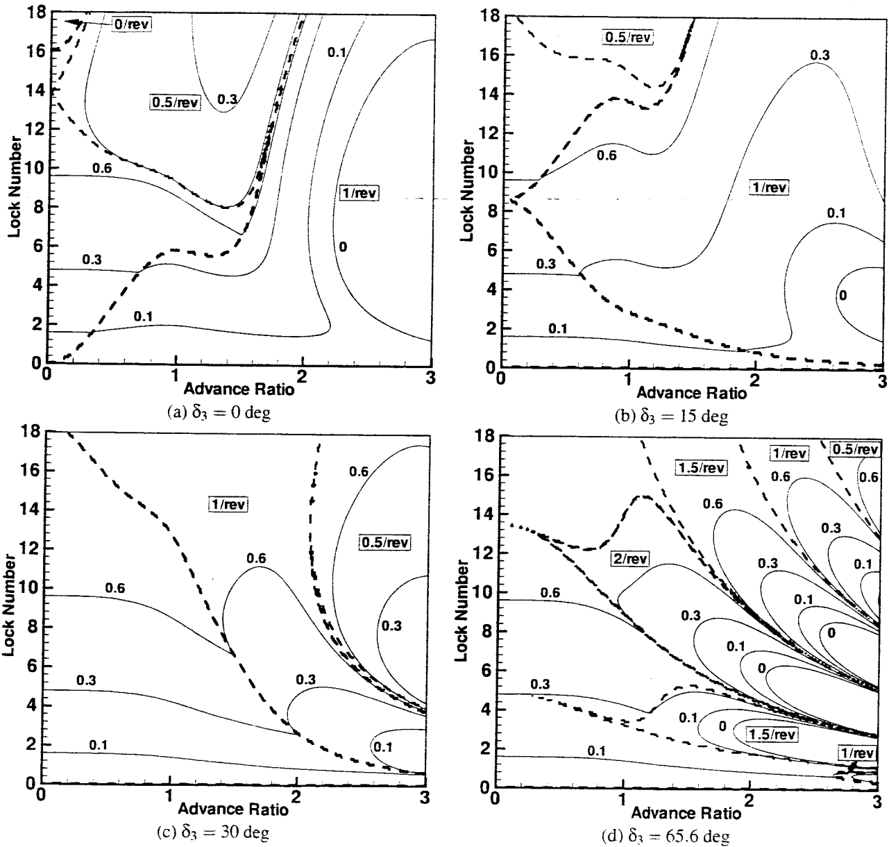
Fig. 1. Stability maps of a rigid blade articulated rotor at 0, 15, 30, and 65.6 deg of \delta_3 , \nu_\beta = 1.0 .
