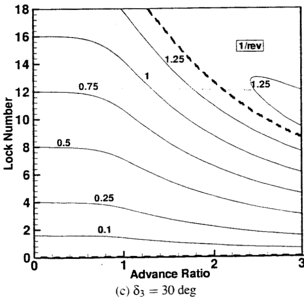
Fig. 2. Stability maps of a rigid blade teetering rotor at 0, 15, 30, and 65.6 deg of \delta_3 .
