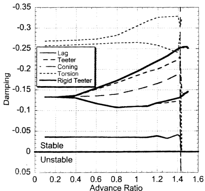
Fig. 33. Stability of elastic teetering rotor at tip speed V_T = 230 ft/sec and torsion frequencies of 8.5/rev.
