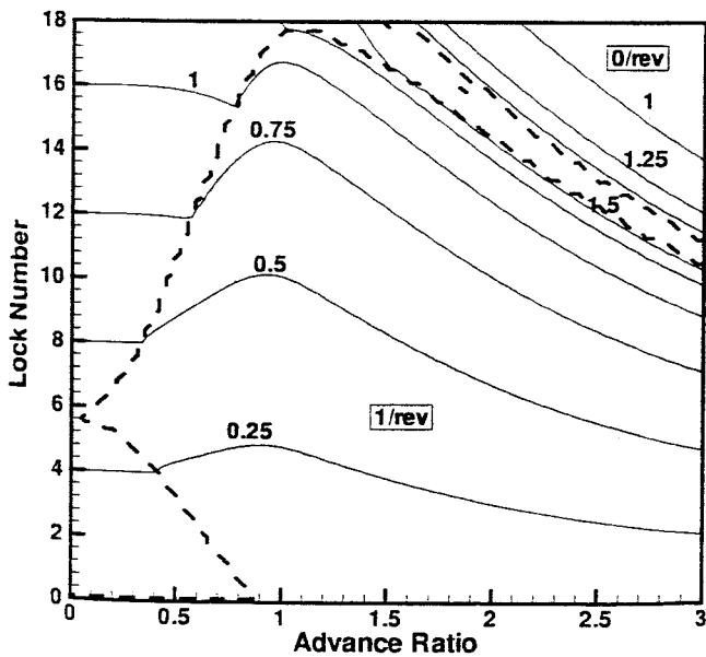
Fig. 7. Stability map for CarterCopter rotor from simplified analysis, \delta_3 = 10 deg, v_\beta = 1.0 ( \gamma \approx 2.5 for CarterCopter).
