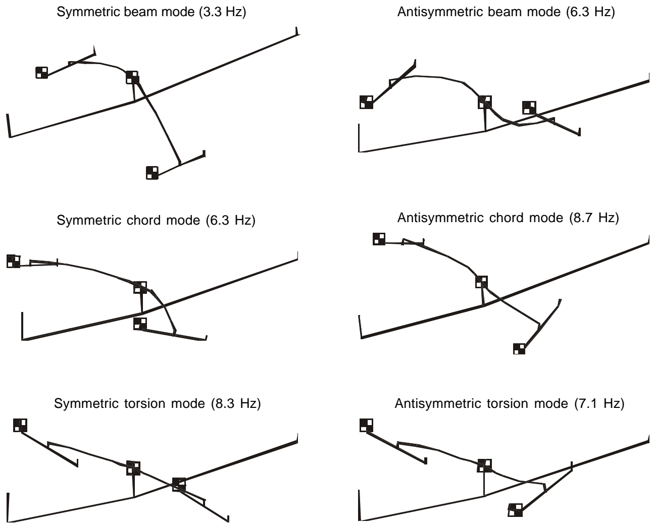
Figure C3. XV-15 stick-model mode shapes and frequencies ( 0.23t/c wing).
