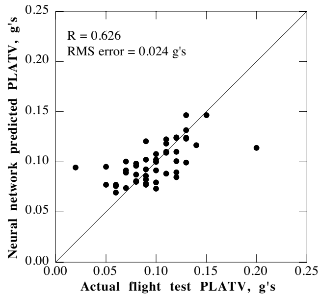
Fig. 5. PLATV correlation using advance ratio and gross weight.
