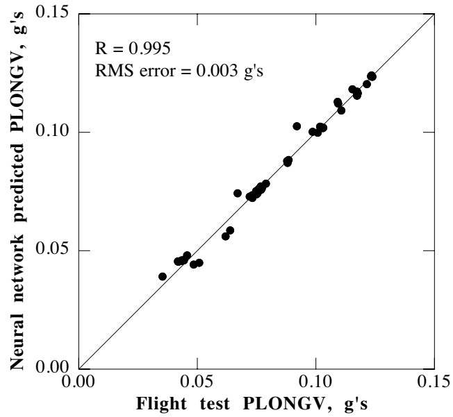
Fig. 18a. PLONGV correlation using wind tunnel rotating system hub accelerations and operating parameters.
