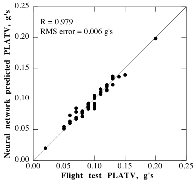
Fig. 14a. PLATV correlation using flight test rotating system hub accelerations and operating parameters.
