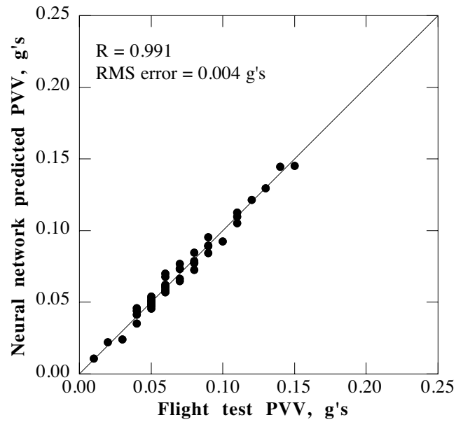
Fig. 13a. PVV correlation using flight test rotating system hub accelerations and operating parameters.
