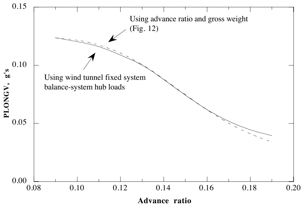
Fig. 21b. PLONGV prediction using six components of N/rev balance-system hub loads and operating parameters ( C_w/\sigma = 0.08 ).
