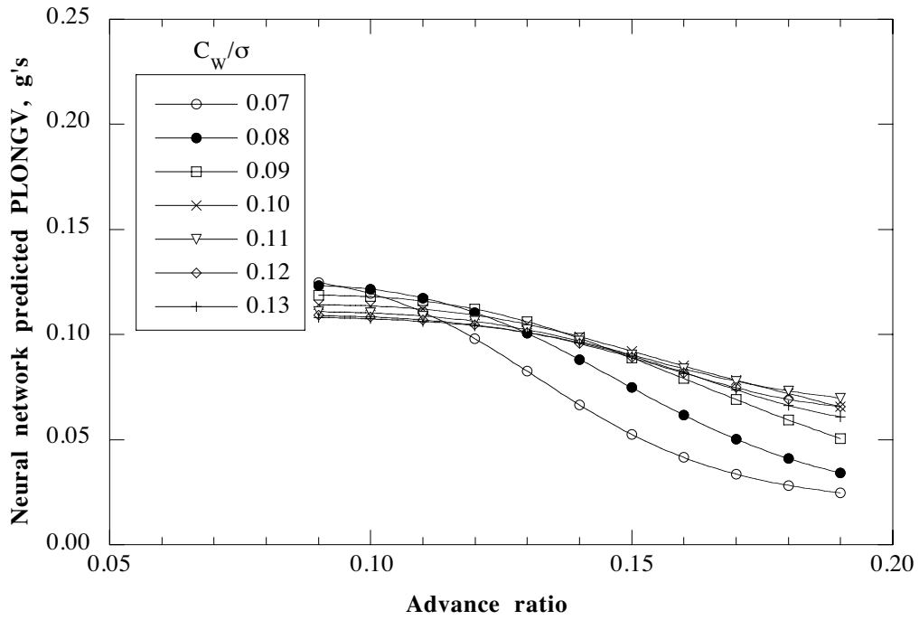
Fig. 9. Predicted PLONGV trends using advance ratio and gross weight.
