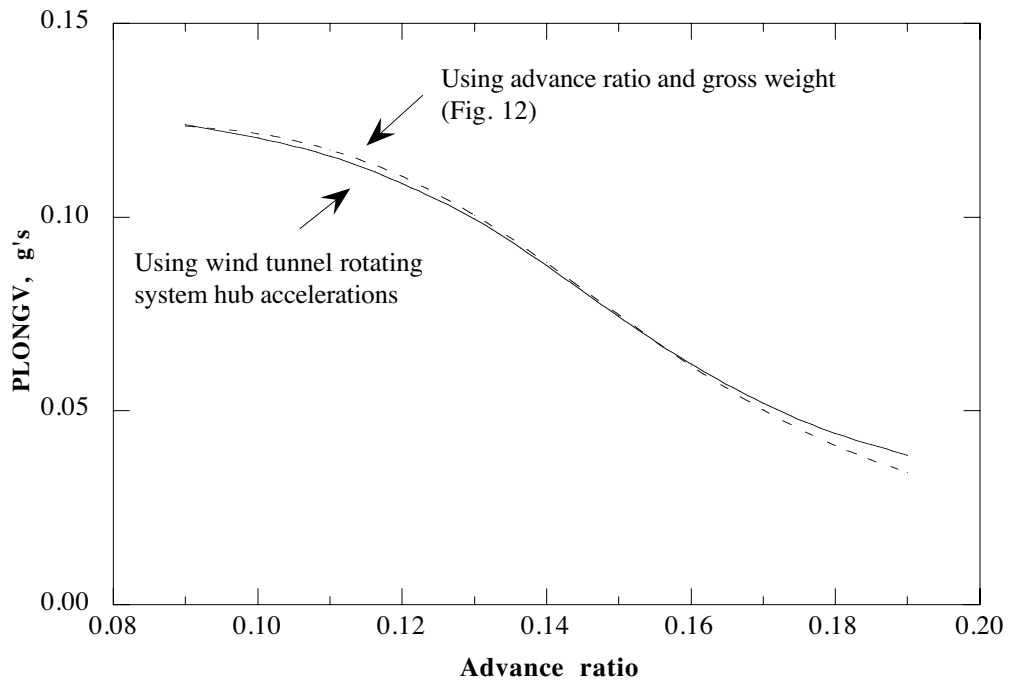
Fig. 18b. PLONGV prediction using wind tunnel rotating system hub accelerations and operating parameters ( C_w/\sigma = 0.08 ).
