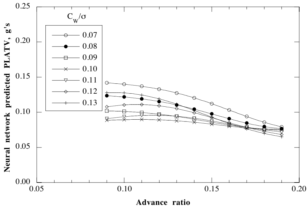
Fig. 8. Predicted PLATV trends using advance ratio and gross weight.
