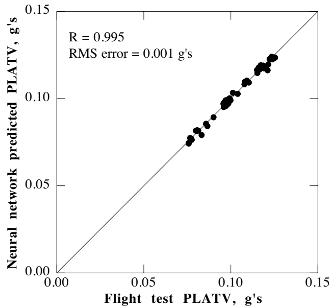
Fig. 20a. PLATV correlation using six components of N/rev balance-system hub loads and operating parameters.
