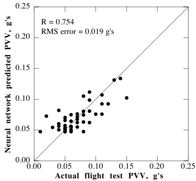
Fig. 4. PVV correlation using advance ratio and gross weight.
