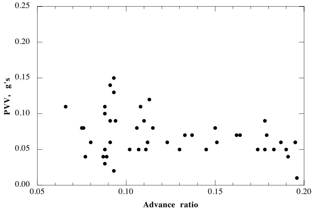
Fig. 1. UH-60A peak, N/rev pilot floor vertical vibration, PVV, variation with advance ratio.
