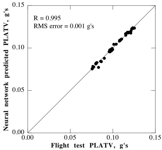
Fig. 17a. PLATV correlation using wind tunnel rotating system hub accelerations and operating parameters.
