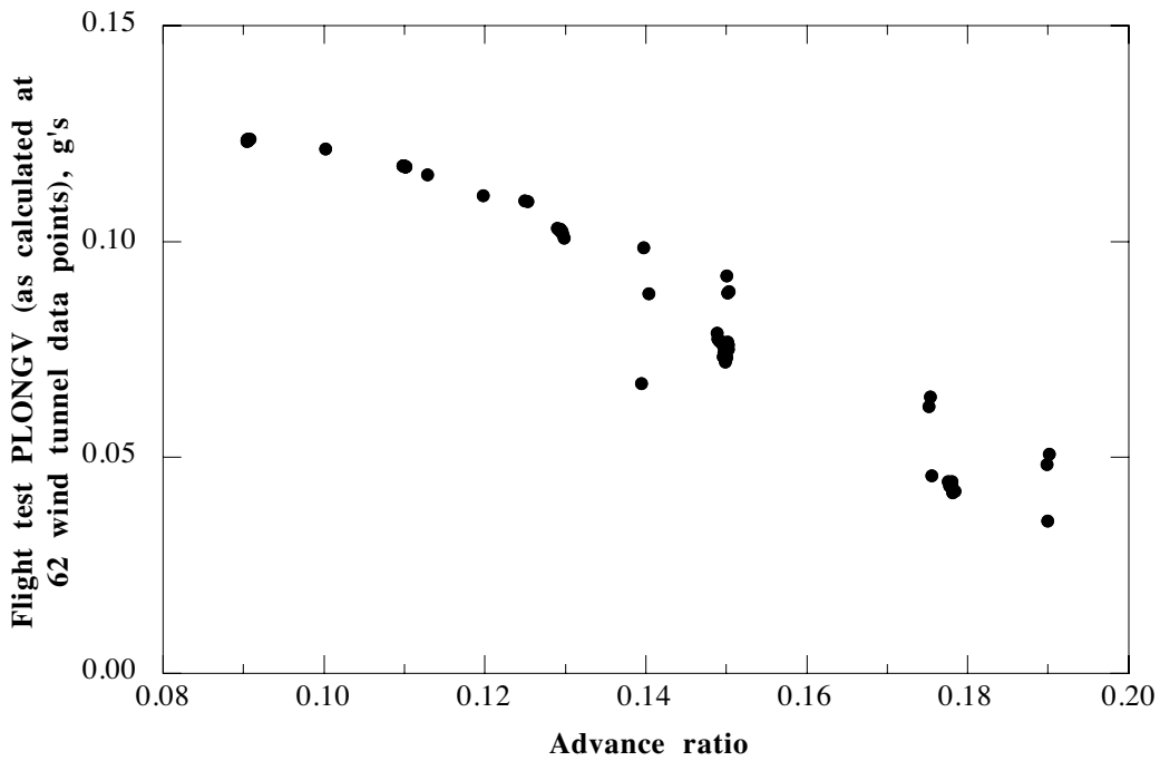
Fig. 12. Predicted flight test PLONGV using advance ratio and gross weight, evaluated at 62 wind tunnel data points, includes thrust variations.
