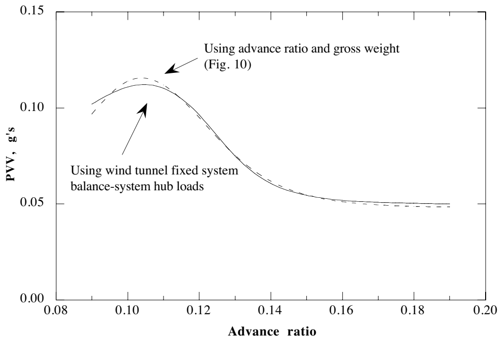
Fig. 19b. PVV prediction using six components of N/rev balance-system hub loads and operating parameters ( C_w/\sigma = 0.08 ).
