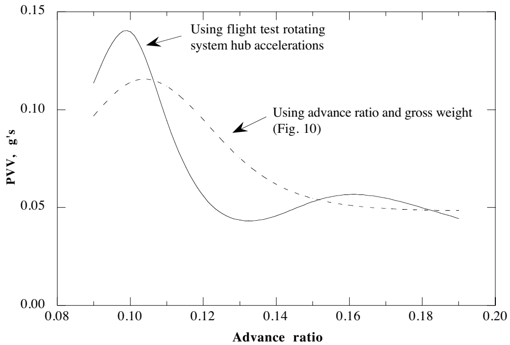
Fig. 13b. PVV prediction using flight test rotating system hub accelerations and operating parameters ( C_w/\sigma = 0.08 ).
