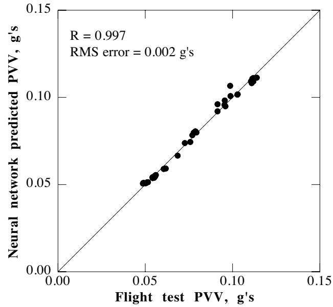
Fig. 16a. PVV correlation using wind tunnel rotating system hub accelerations and operating parameters.
