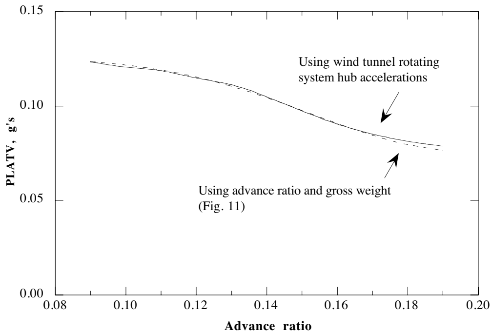
Fig. 17b. PLATV prediction using wind tunnel rotating system hub accelerations and operating parameters ( C_w/\sigma = 0.08 ).
