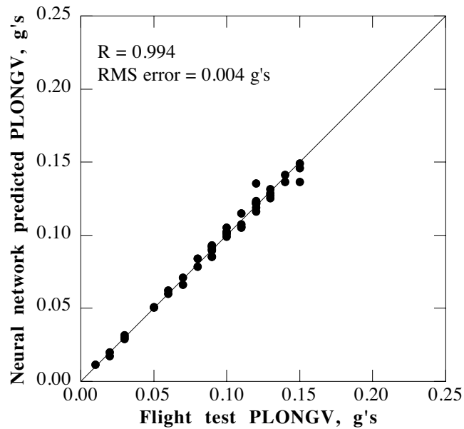
Fig. 15a. PLONGV correlation using flight test rotating system hub accelerations and operating parameters.
