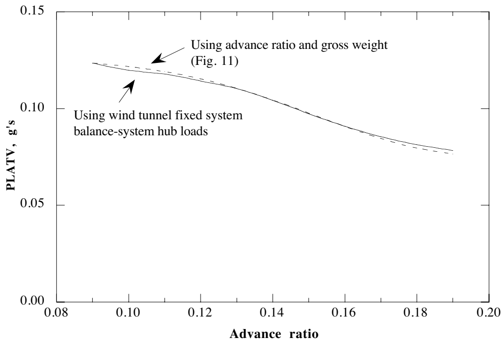
Fig. 20b. PLATV prediction using six components of N/rev balance-system hub loads and operating parameters ( C_w/\sigma = 0.08 ).
