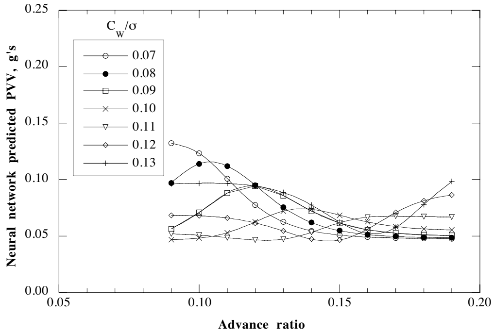
Fig. 7. Predicted PVV trends using advance ratio and gross weight.
