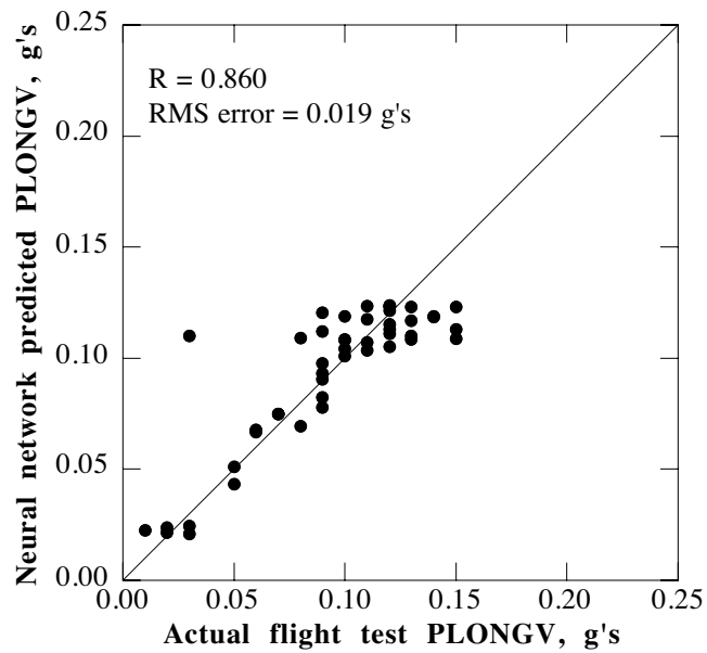
Fig. 6. PLONGV correlation using advance ratio and gross weight.
