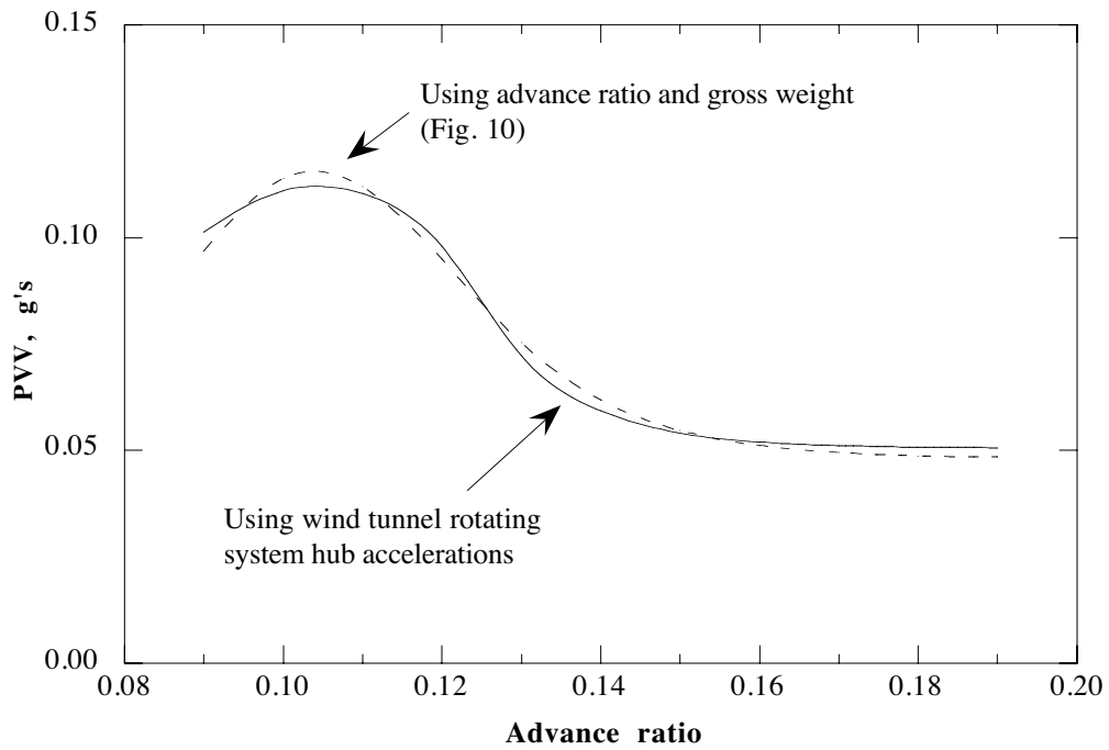
Fig. 16b. PVV prediction using wind tunnel rotating system hub accelerations and operating parameters ( C_w/\sigma = 0.08 ).
