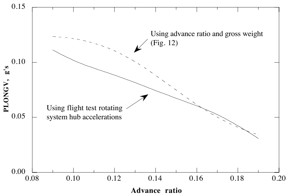
Fig. 15b. PLONGV prediction using flight test rotating system hub accelerations and operating parameters ( C_w/\sigma = 0.08 ).
