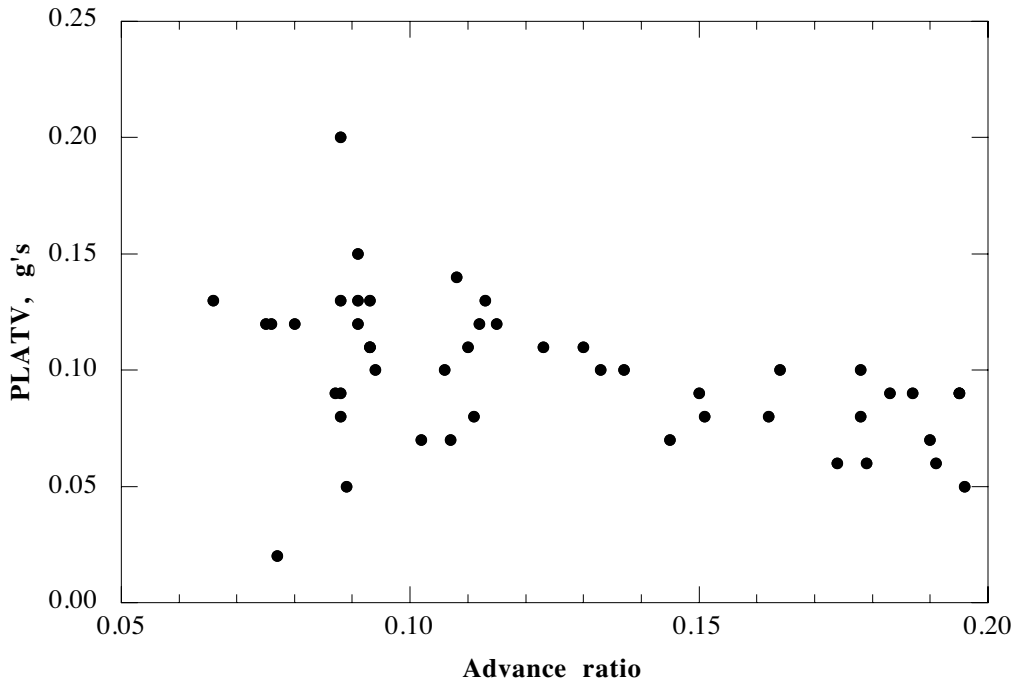
Fig. 2. UH-60A peak, N/rev pilot floor lateral vibration, PLATV, variation with advance ratio.
