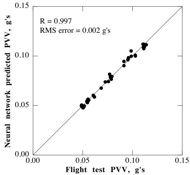
Fig. 19a. PVV correlation using six components of N/rev balance-system hub loads and operating parameters.
