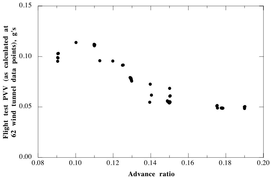
Fig. 10. Predicted flight test PVV using advance ratio and gross weight, evaluated at 62 wind tunnel data points, includes thrust variations.
