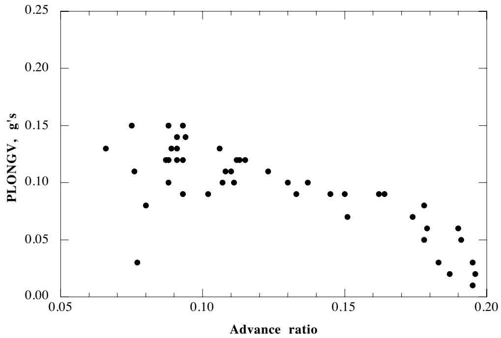
Fig. 3. UH-60A peak, N/rev pilot floor longitudinal vibration, PLONGV, variation with advance ratio.
