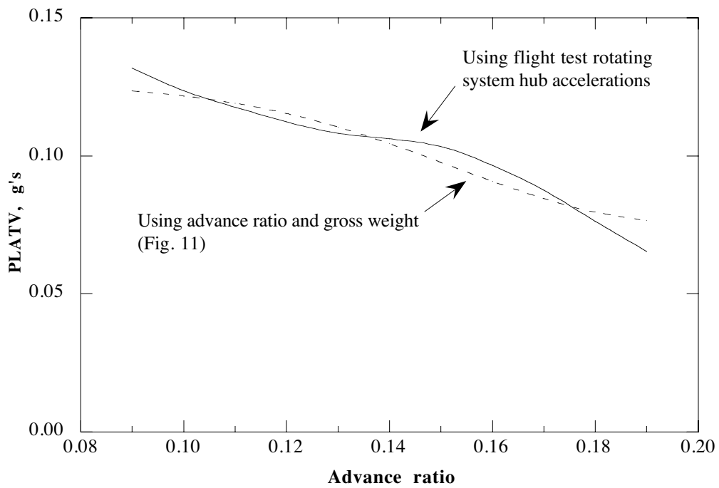
Fig. 14b. PLATV prediction using flight test rotating system hub accelerations and operating parameters ( C_w/\sigma = 0.08 ).
