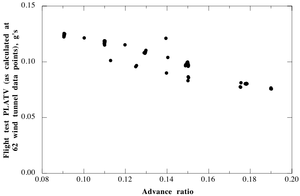
Fig. 11. Predicted flight test PLATV using advance ratio and gross weight, evaluated at 62 wind tunnel data points, includes thrust variations.
