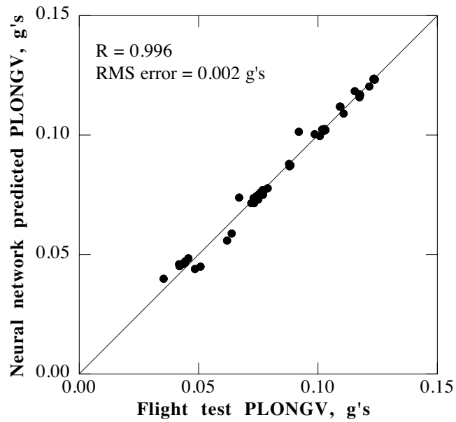
Fig. 21a. PLONGV correlation using six components of N/rev balance-system hub loads and operating parameters.
