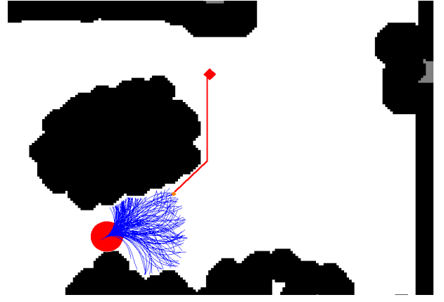
Fig. 2. Navigation planner view showing local candidate curves in blue and the straighter global D* path (in red) connecting the best local path to the goal (red diamond). Obstacles are in black.
