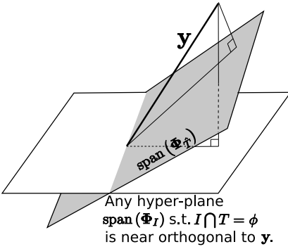
Figure 5. Correlation maximization works in the SP setting.
