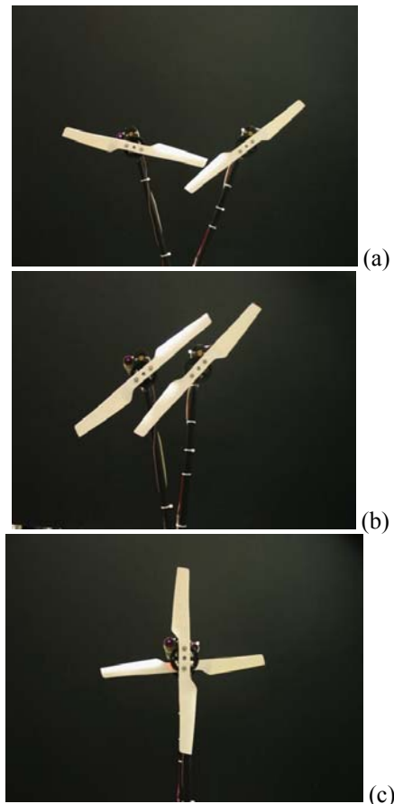
Fig. 35 – Examples of Unducted Rotor Configurations ( h/R = 0.617 ): (a) s/R = 0.69 , (b) s/R = 0.345 , and (c) s/R = 0
