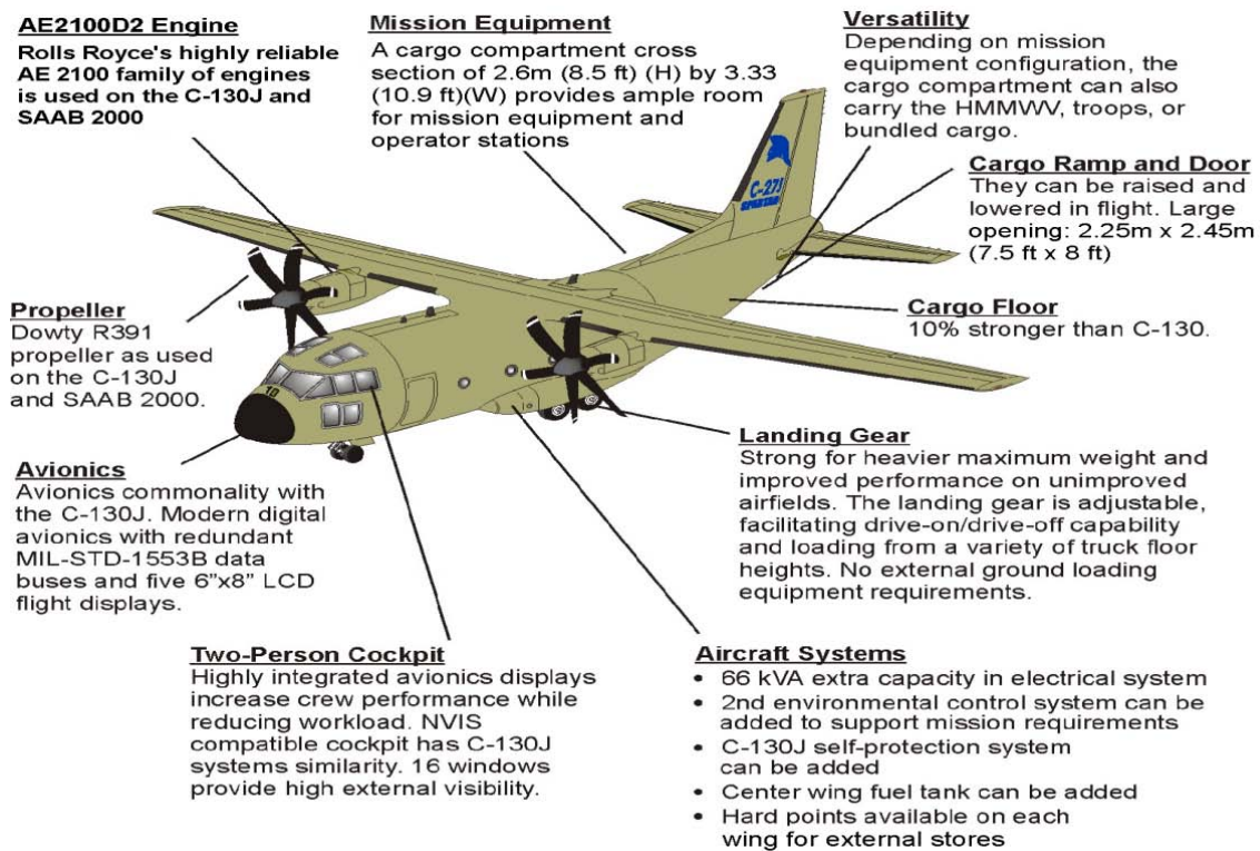
Figure 5. The C-27J Spartan.
