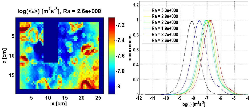
Figure 3. A - Time-averaged TKED rate ( m^2 s^{-3} ) map at Ra=2.6 \cdot 10^8 B- histogram of TKED rates for different Ra numbers. Note the TKED distribution follows Gaussian around the TKED peak.
