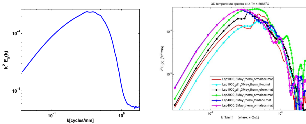
Figure 5. Three dimensional temperature dissipation spectra – k^2 * E_\theta(k) .
