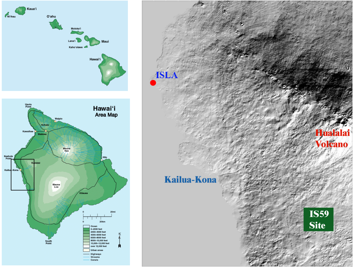
Figure 1. Location of IS59 and Infrasound Laboratory (ISLA) on the island of Hawaii.
