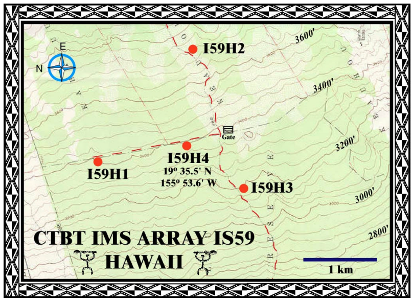
Figure 2. Infrasonic array geometry.
