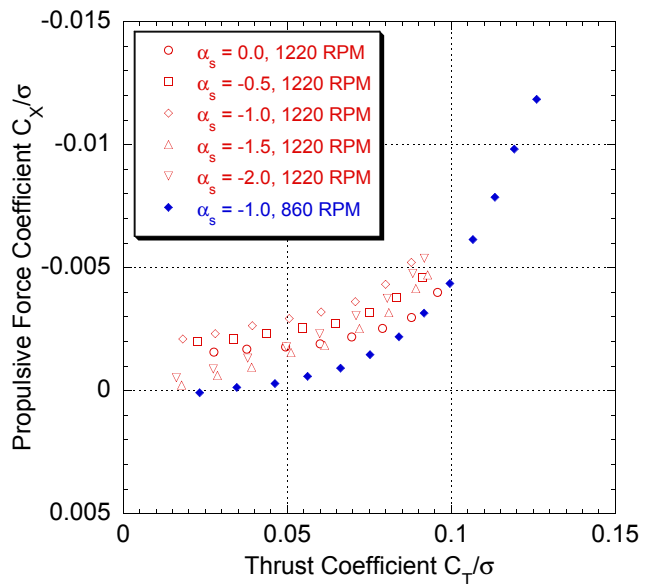
Fig. 12. Propulsive force vs. thrust at advance ratio \mu = 0.25 , shaft angles -2 \leq \alpha_s \leq 0 deg, 1220 and 860 RPM.
