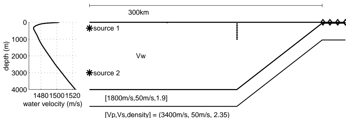
Figure 1 Environmental model for PE computations. The water velocity profile used for all computations is shown at left. The diamonds denote seismometer locations, recording vertical displacement, and the asterisks denote the 2 source locations used in the modeling. The position of a vertical hydrophone array is marked by the dotted line.
