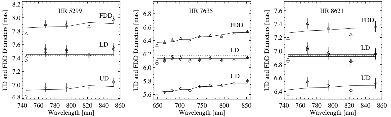
Fig. 5. Diameters based on uniform disk (UD, diamonds) and fully darkened disk (FDD, triangles) models for each spectral channel together with the Kurucz model atmosphere predictions (connected by solid lines). In addition, the limb-darkened (LD) diameters are shown which were derived by applying correction factors to the UD and FDD diameters. The mean LD diameters as quoted in Table 2 are indicated by the solid lines. The error bars represent the standard deviation of the obtained LD diameters. For comparison, the dotted lines indicate the limb-darkened diameters which were derived by the direct fit to a grid of Kurucz model atmospheres.
