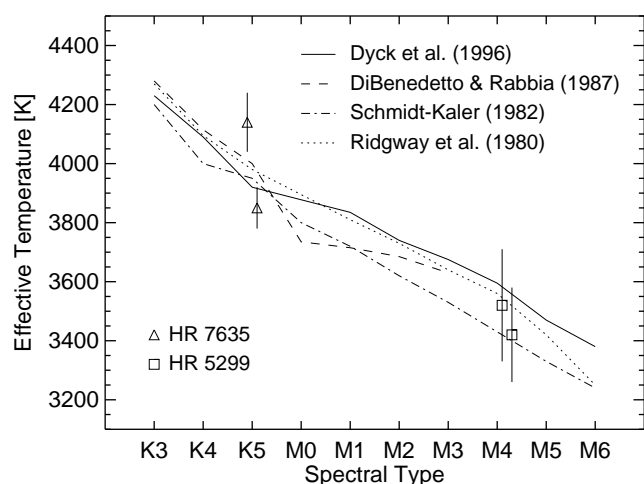
Fig. 7. Comparison of our derived HR 5299 and HR 7635 T_{\text{eff}} values with different effective temperature scales (Ridgway et al. 1980, Schmidt-Kaler 1982, DiBenedetto & Rabbia 1987, Dyck et al. 1996). The symbols shifted to the left of the nominal spectral type position indicate the values derived by the direct fit to a grid of Kurucz model atmospheres. The symbols shifted to the right indicate the values derived from the limb-darkened angular diameter \Theta_{\text{LD}} and the bolometric flux F_{\text{bol}} .
