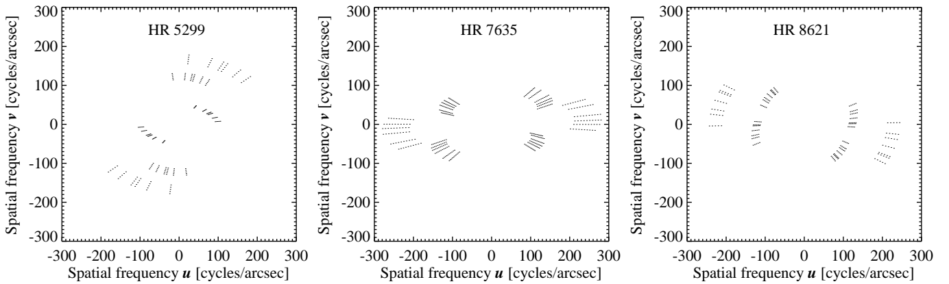
Fig. 1. Plot of the obtained coverages of the uv -plane of the HR 5299, HR 7635 and HR 8621 observations based on all observation dates (see Table 1) and on those spectral channels which were used for the data analysis, i.e. the 10 reddest channels for HR 7635 and the 5 reddest channels for the fainter stars HR 5299 and HR 8621.
