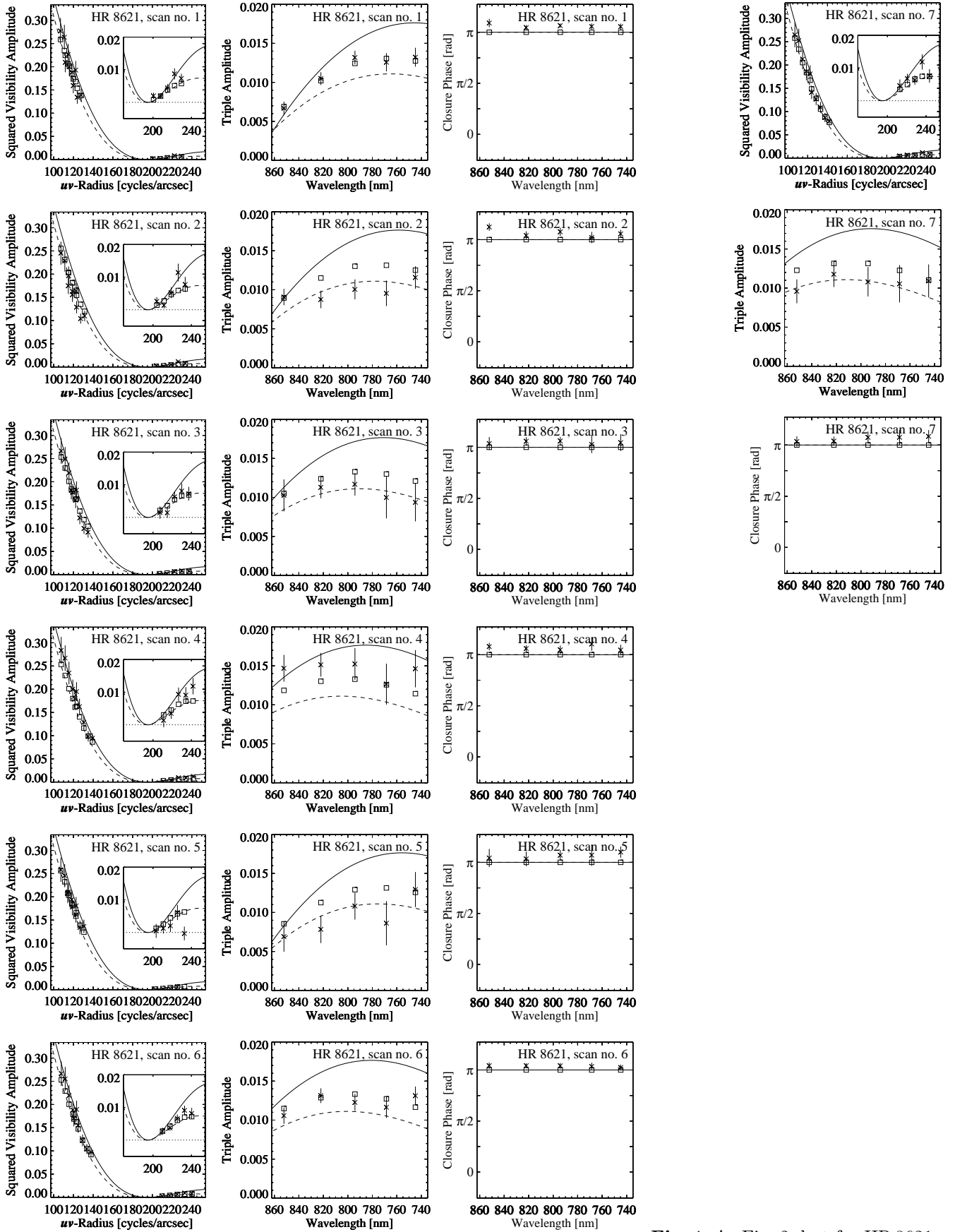
Fig. 4. As Fig. 2, but for HR 8621.
