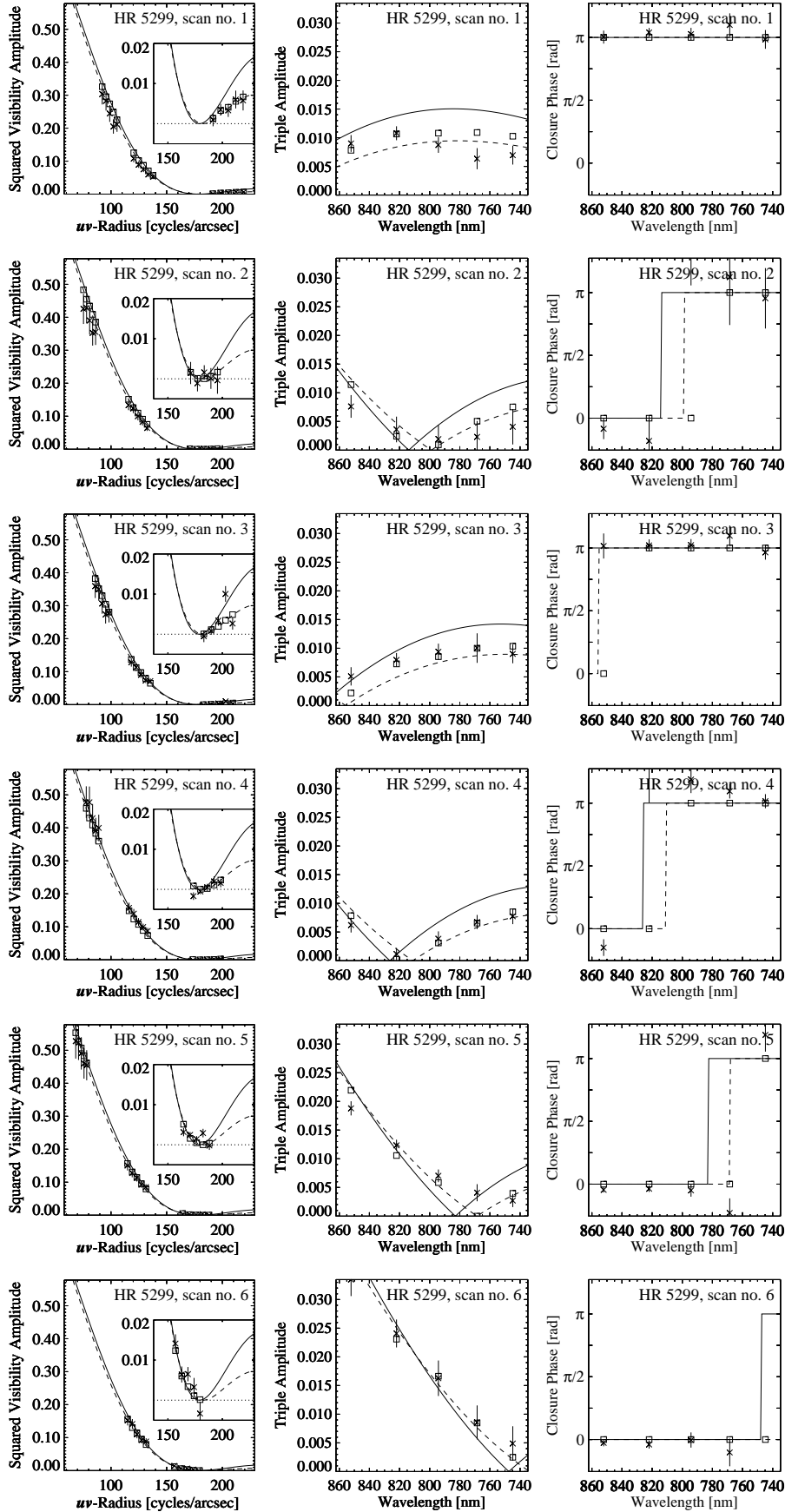
Fig. 2. Squared visibility amplitudes (left), triple amplitudes (middle), and closure phases (right) of HR 5299 and of best fitting models, for all obtained scans. The squared visibility amplitudes are plotted as a function of the uv -radius, and the triple amplitudes and closure phases as a function of the spectral channels' central wavelengths. The inset plots (left) provide an enlarged view of the low squared visibility amplitude values around and beyond the first minimum. The x-symbols with error bars indicate the observations and their errors, the solid line the model values based on a uniform disk, the dashed line those based on a fully darkened disk, and the squares those based on the best fitting Kurucz stellar model atmosphere (Kurucz 1993). The error bars include the formal errors as well as the calibration errors as described in Sect. 3.
