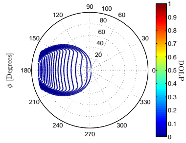
(a) DOLP of Al, 2^{1/2}\sigma_h/\ell = 0.1 .
