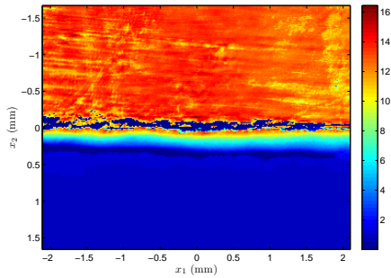
(c) Painted Al, turbulence-degraded \kappa .
