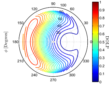
(f) DOLP of glass, 2^{1/2}\sigma_h/\ell = 0.6 .
