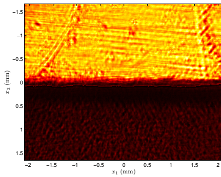
(e) Painted Al, corrected S_0 .
