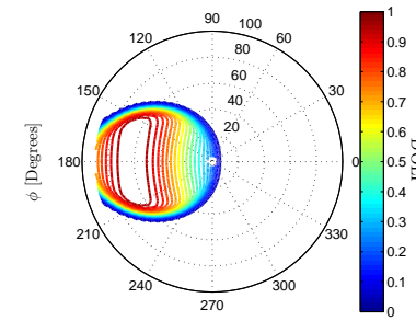
(g) DOLP of Teflon, 2^{1/2}\sigma_h/\ell = 0.1 .
