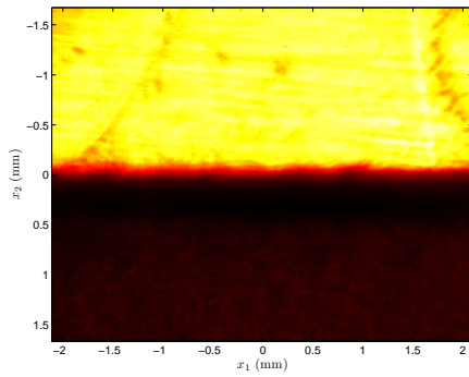
(c) Painted Al, turbulence-degraded S_0 .
