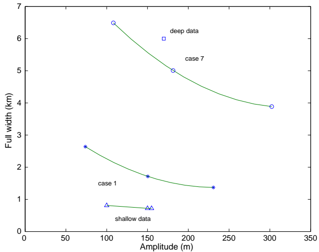
Fig. 23. Dispersion of full width ( 2L ) versus amplitudes for case 1 (star), case 7 (open circle), thermistor chain data (triangle) at mooring S7 in 350 m depth and deep water measurements west of Luzon Strait (square). Lines indicate a least square polynomial fit.
