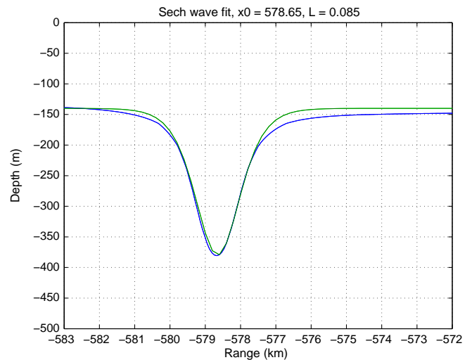
Fig. 24. \text{Sech}^2 analytical KdV solution fit (green curve), to the \sigma_\theta = 25.05 isopycnal at 74 h in case 1 (blue curve). (For interpretation of references in color in figure legends, the reader is referred to the web version of this article.)
