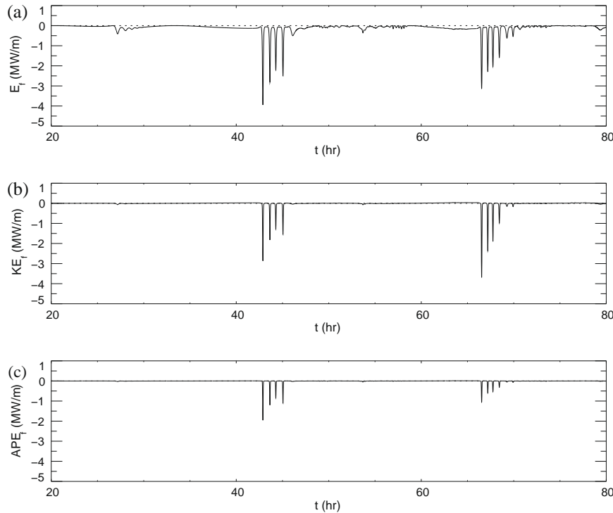
Fig. 17. Energy fluxes at x = -200 km for case 1: (a) linear energy flux, (b) kinetic energy flux and (c) available potential energy flux.
