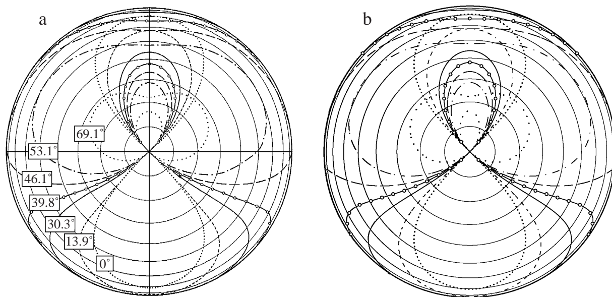
Figure 4. (a) Neutral lines (contours of polarization directions at \pm 45^\circ to the vertical), calculated by multiple-scattering theory [8], for the indicated Sun elevations; (b) neutral lines for the same Sun elevations as in (a), calculated on the simple theory based on (2.7) and (5.1) with the same locations of the singularities as in (a). The circles are almaccantars (loci of constant elevation), spaced at 10^\circ intervals; radial distance is proportional to \cos(\text{elevation angle}) .
