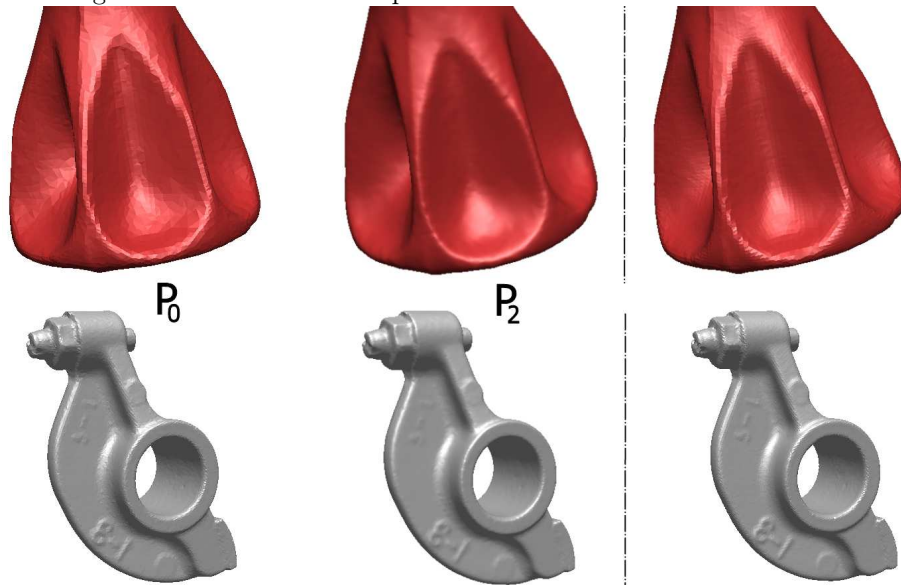
Fig. 9. Flatly shaded renderings of the surfaces reconstructed from the non-simplified Youthful point set (left) and P_2 of Figure 8 illustrating how meshless subdivision of a base point set resulting from point cloud simplification may be used to obtain a smoother, more regular and more compact representation of the original data set of 1728305 points.
