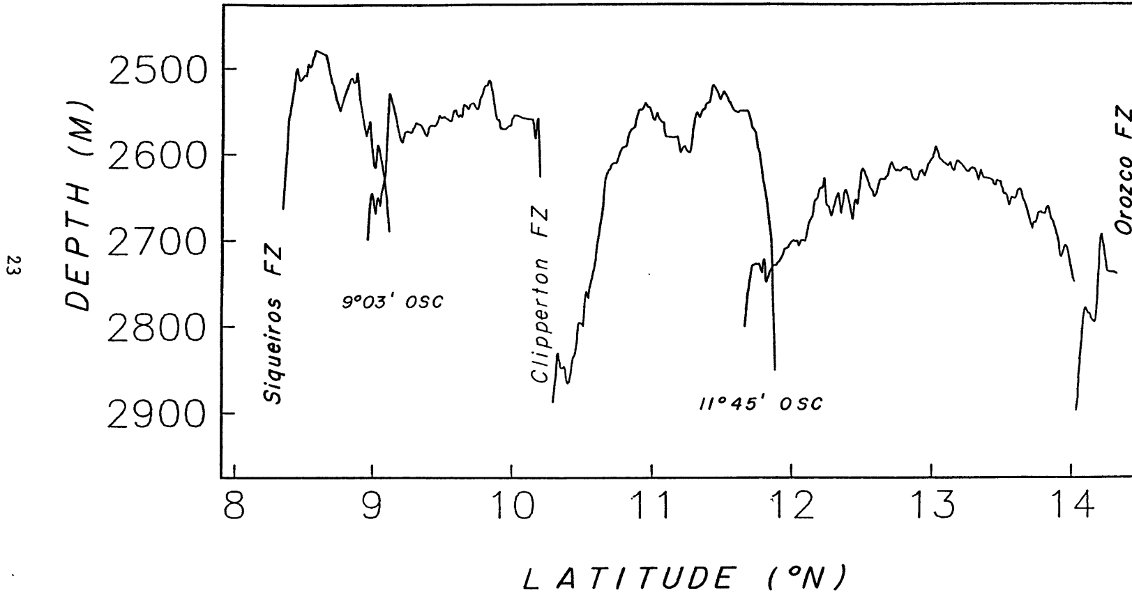
1.2 Along-strike axial depth profile of East Pacific Rise segments projected onto a single plane. Ridge discontinuities at fracture zones and large offset OSCs are labeled.
