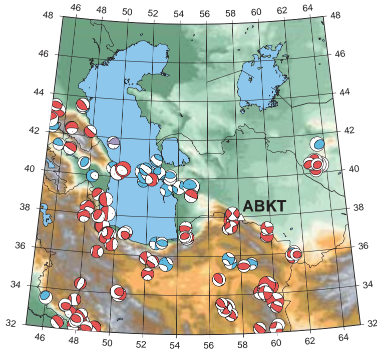
Figure 2. Location of station ABKT at Alibek, Turkmenistan (37.9304N, 58.1189E, 678 m), shown with topographic variations and focal mechanisms from the Harvard CMT catalog. Mechanisms are shaded by depth (red indicated depths from 0 to 32 km; blue depths from 33 to 70 km; and purple depths greater than 70 km).
