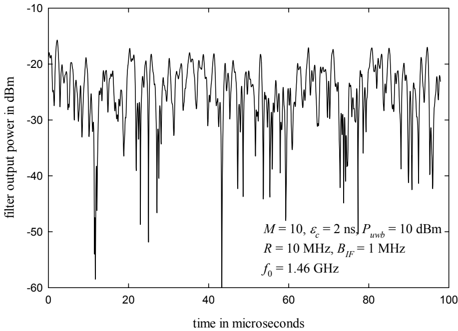
Figure 5-12: Simulation output for 1.46 GHz, which has a small spectral line
