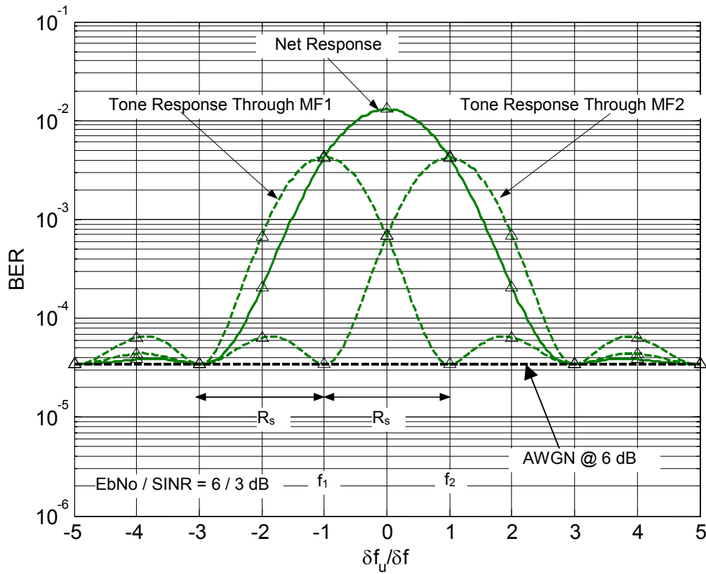
Figure 7-11: BER using UWB Tone Model; Shows tone response through each branch separately; I/N=6 \text{ dB}
