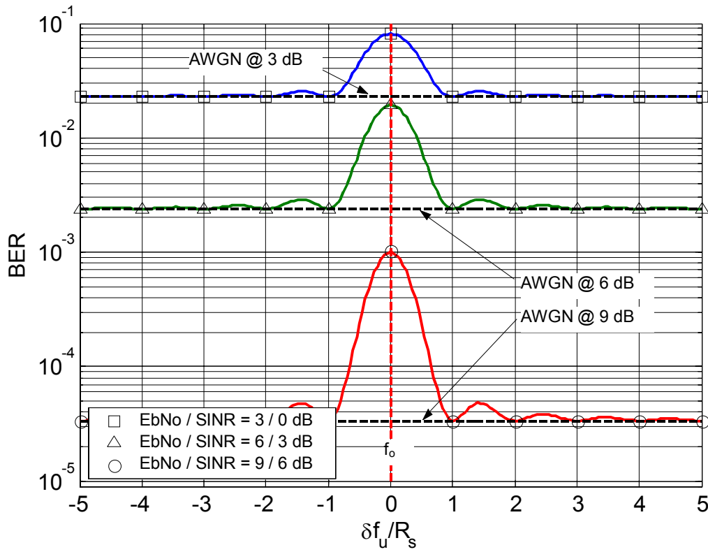
Figure 6-10: BER using UWB Tone Model; Performance as a function of spectral line location; I/N=0 \text{ dB}
