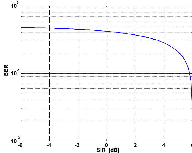
Figure 8-3: BER versus SIR for the case of high E_b/N_o .
