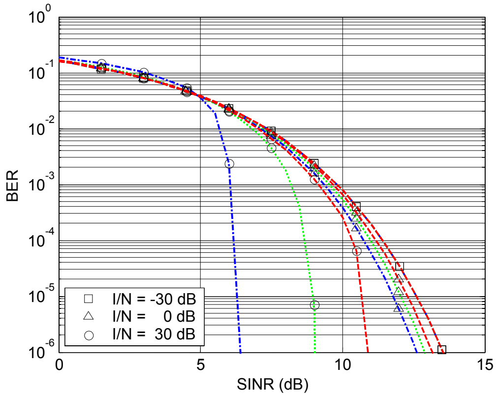
Figure 7-8: BER performance using UWB Pulse model; Dashed-dotted blue line ( N_u = 1 ), Dotted green line ( N_u = 5 ), Dashed red line ( N_u = 10 )
