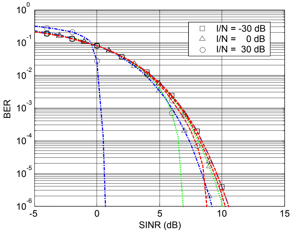
Figure 6-8: BER performance using UWB Pulse model; Dashed-dotted blue line ( N_u = 1 ), Dotted green line ( N_u = 5 ), Dashed red line ( N_u = 10 )
