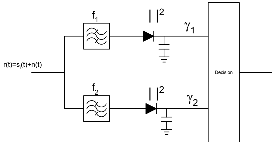
Noncoherent FSK Detector
