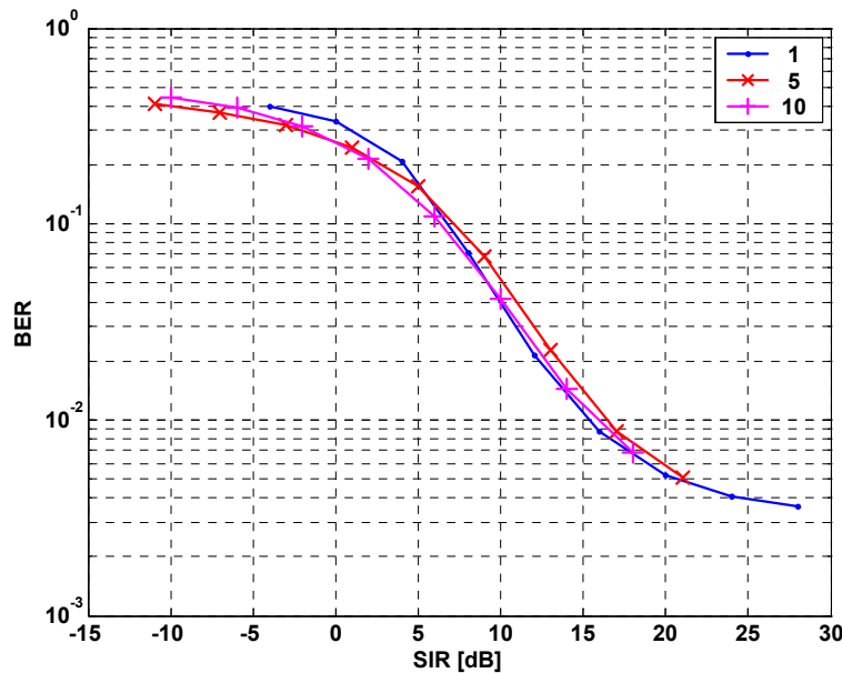
Figure 8-7: BER versus SIR with varying number of interfering pulses N_u with E_b/N_o=10 dB
