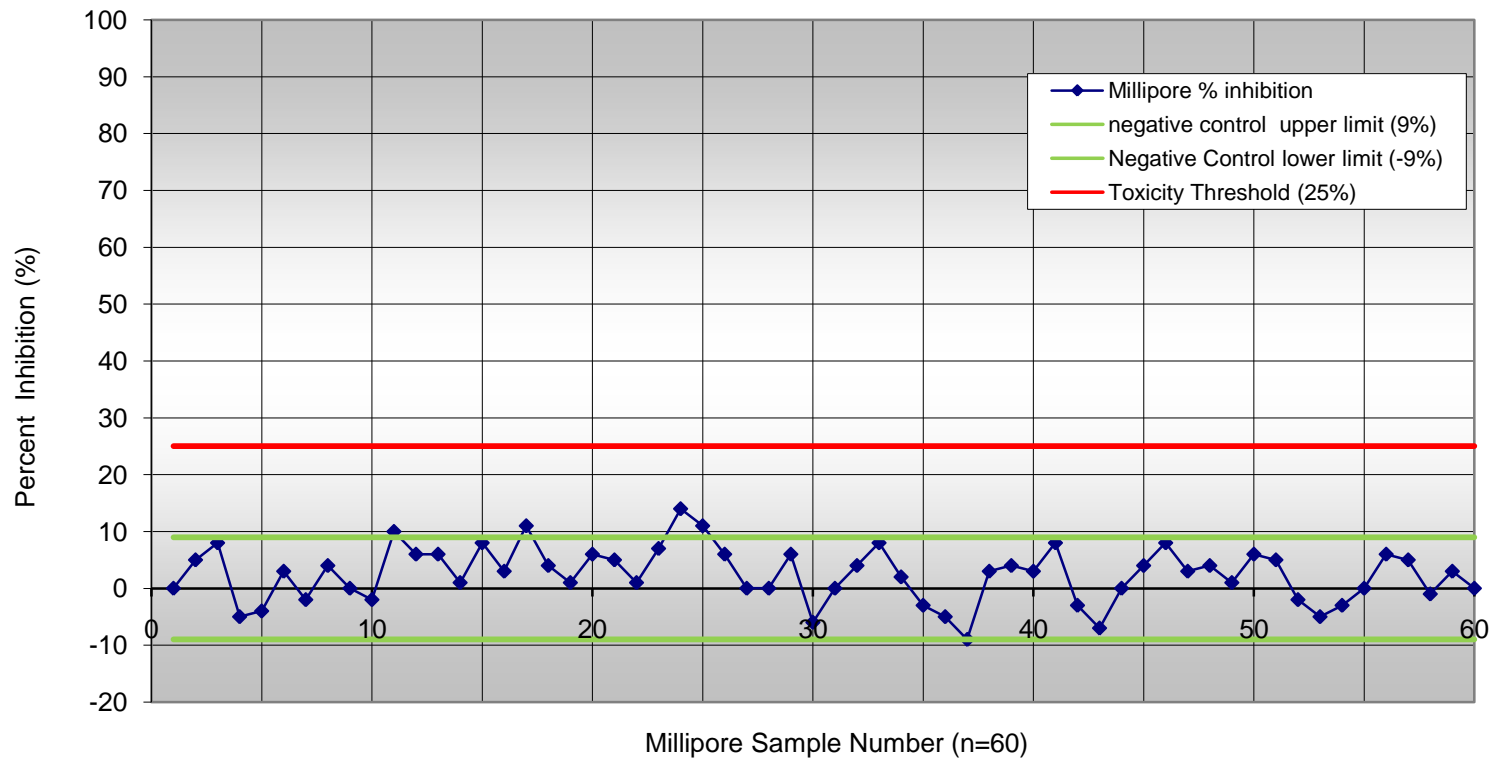
Figure 3-1. Eclox Chemiluminescence Negative Controls. Four of the 60 control samples exceeded 9% inhibition. A red reference line is provided at 25% inhibition, the minimum level established for a positive response.
