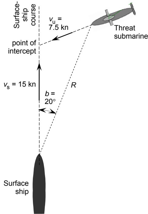
Figure 2: Schematic diagram of the scenario used in the calculation of cumulative detection probabilities
