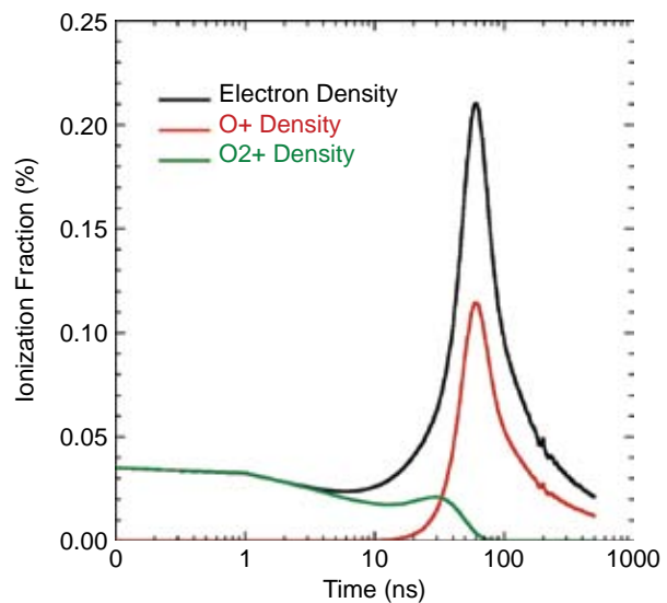
FIGURE 8 Enhancement of an air plasma by a 50-ns, 1-Joule laser pulse. As the air is heated, avalanche ionization overcomes the losses, and the electron density increases. Molecular dissociation can also be seen.
