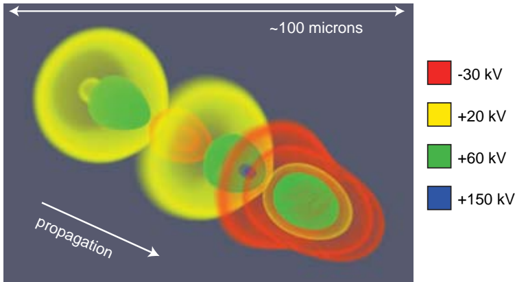
FIGURE 6 The scalar potential in a laser wakefield accelerator as computed by turboWAVE. The structure is in motion at the speed of light. The high potential gradients lead to the rapid acceleration of electrons to high energies.
