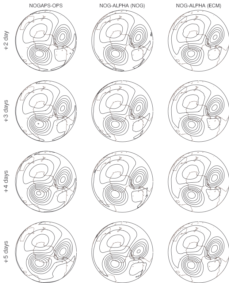
FIG. 8. Geopotential height at 10 hPa (~32 km) over the SH for forecasts evaluated at 25 September 2002. The left column is the NOGAPS operational analysis, the middle column is NOGAPS- \alpha (nog), and the right column is NOGAPS- \alpha (ecm). The length of forecast is provided on the left hand side. Contour interval is 400 m.
