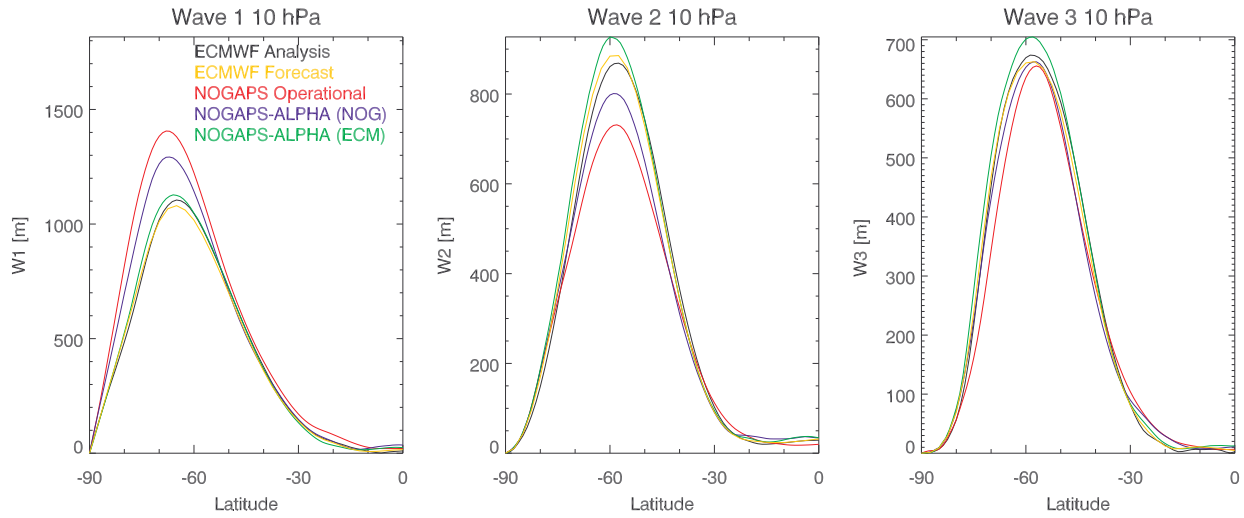
FIG. 3. Geopotential height zonal wave 1, 2, and 3 amplitudes at 10 hPa (~32 km) over the SH for 5-day forecasts initialized 20 September 2002. The colors determine the particular run, as indicated in the first plot.
