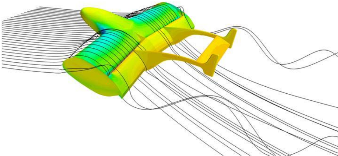
Figure 39. Numerical CFD Simulation of the Propulsive Wing UAV at High AOA. From [5]
