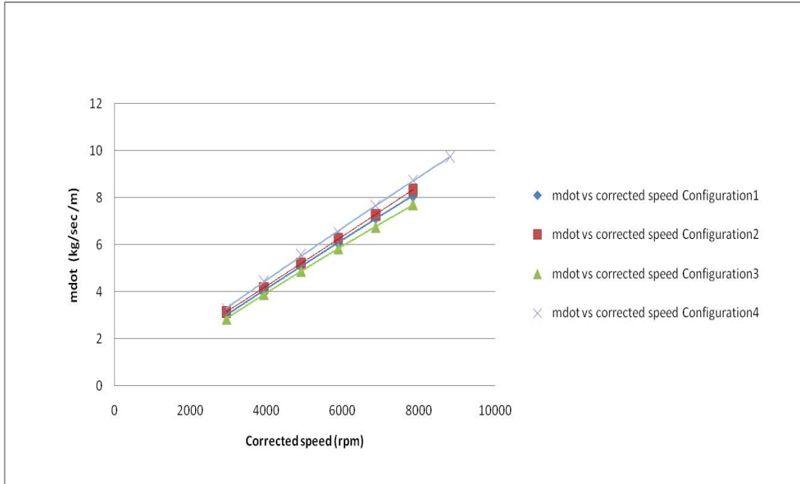
Figure 13. Numerical CFD Results for \dot{m} dot (kg/sec/m) vs. Corrected Speed
