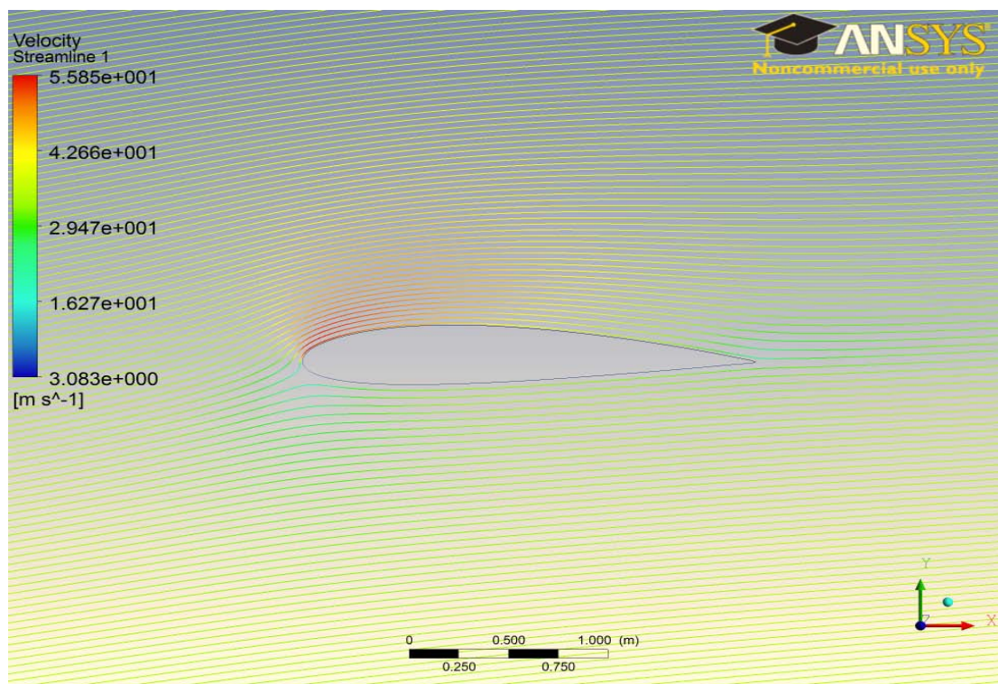
Figure 31. Streamlines for NACA 2415 at AOA 8°, c = 2.28\text{m} , U = 3.5\text{ m/s}
