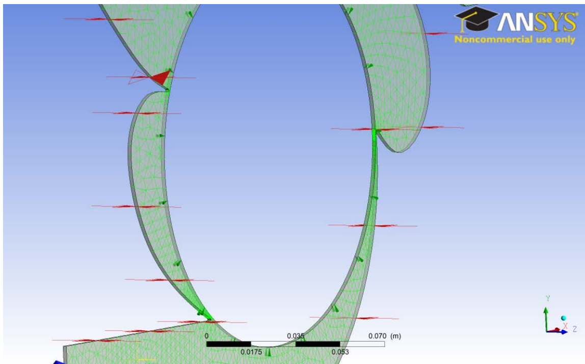
Figure 6. Two-Dimensional (2-D) Meshing (Casing 8,747) in ANSYS CFX Mesh Tool, Without Inflated Layers
