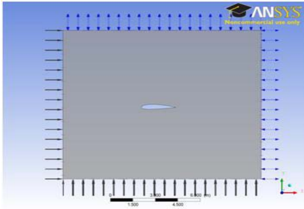
Figure 30. Boundary Conditions Specification with CFX-Pre of the NACA 2415 Airfoil
