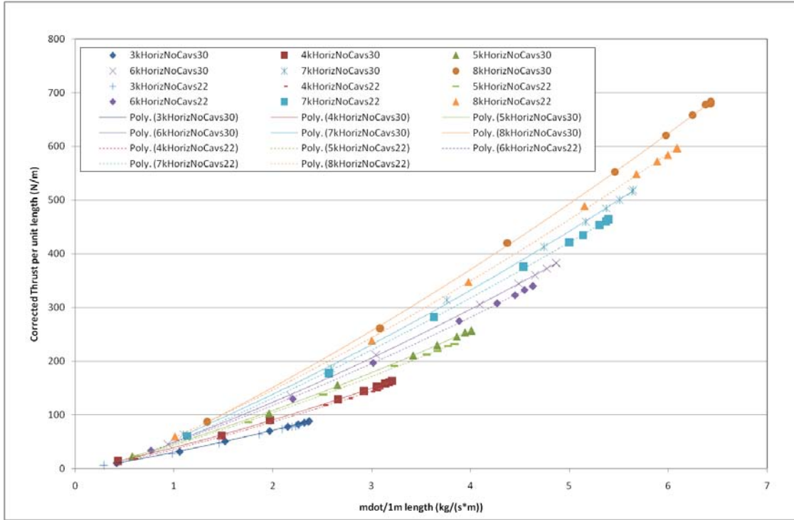
Figure 42. Test Plan A Experimental Results for Corrected Thrust per Unit Length
