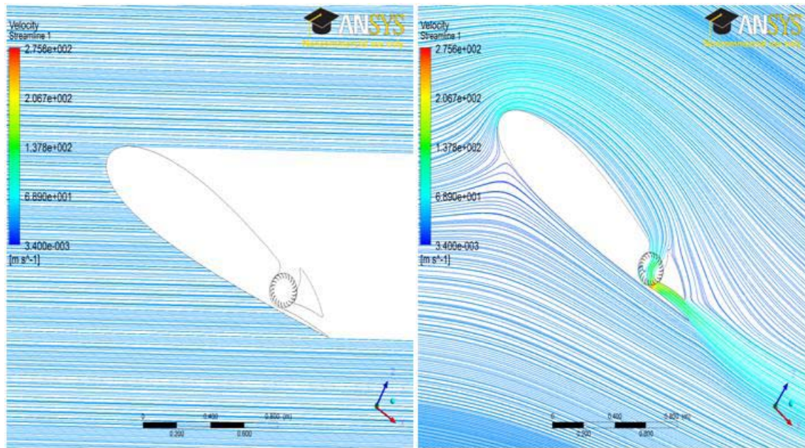
Figure 38. Propulsive Wing NACA 2421 at 30^\circ AOA, Fully Embedded 22-Bladed Rotor CFF (a) Initial Time Step Streamlines, (b) Steady-State' Time Step Streamlines, CFF On
