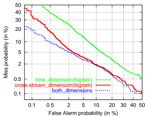
Figure 5: Combination of the Cross-stream Dimension (bigram) with the Time Dimension (bigram)
