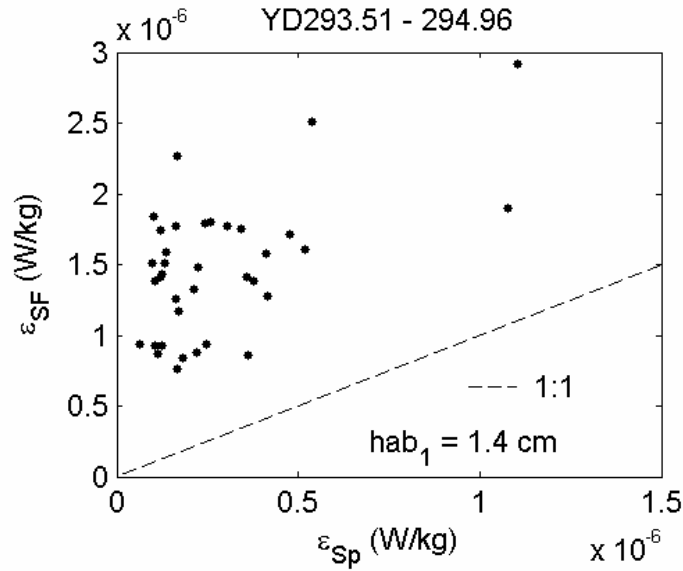
Figure 1. Turbulent kinetic energy dissipation rates near the bed in the presence of relict ripples following Tropical Storm Matthew.
