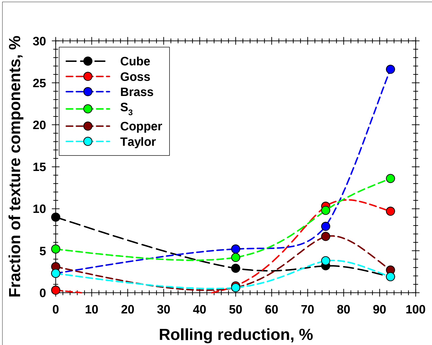
Figure 8. The evolution of rolling-texture components (within 15^\circ of the ideal orientations) as a function of the rolling reduction.
