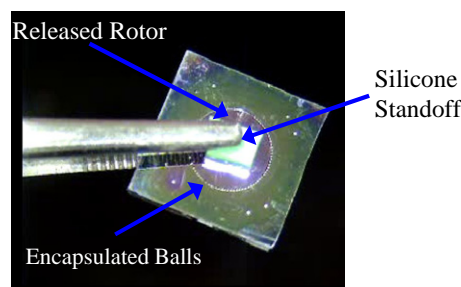
Figure 5. Optical picture of a released silicon rotor supported by stainless steel balls at the periphery. A full compliment configuration was used with more than 60 balls.
