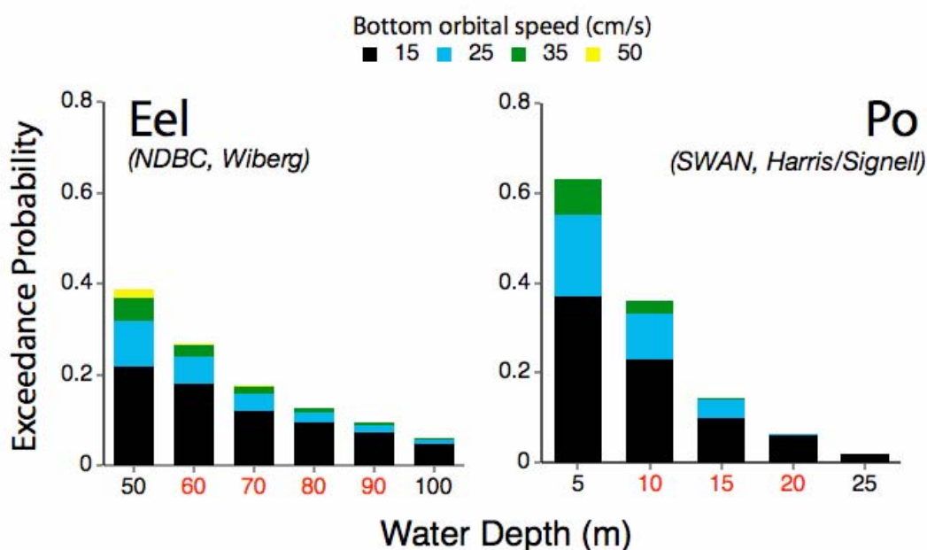
Figure 2. The exceedance probability of bottom orbital speeds (15, 25, 35 & 50 cm/s) as a function of depth for the Eel and Po river margins. The Eel estimates were made by Patricia Wiberg (UVa) using NOAA-NDBC data, whereas the Po estimates were made by Courtney Harris (VIMS) and Rich Signell (USGS) using modeled wind. In both panels, the depth of the flood deposits is depicted in red.
