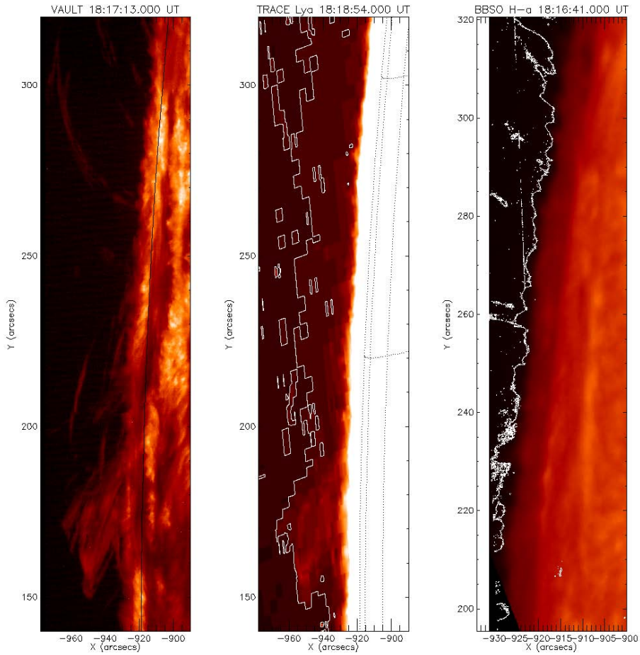
Figure 4. VAULT-II, TRACE Ly \alpha , and BBSO H \alpha comparison of the solar limb. All intensities are individually trimmed and scaled to emphasize the fainter details. Left: VAULT-II after alignment and calibration. The black contour follows the visible limb, as aligned with the TRACE White light channel. Center: TRACE Ly \alpha . The black grid denotes the photosphere. The prominence is much fainter than in the VAULT images but it is still visible. The white contour close to noise level helps to correlate with VAULT. Right: H \alpha channel from ground-based BBSO. The BBSO FOV is slightly smaller than the other instruments. The dotted contour denotes the VAULT edge. Note that the H \alpha spicule heights are up to \sim 2'' shorter than in Ly \alpha .
