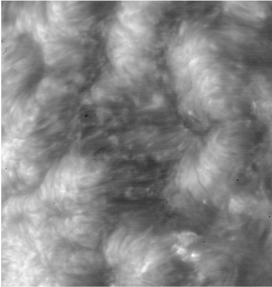
Figure 8. Detail of a supergranular cell in the Quiet Sun in \text{Ly}\alpha . The horizontal extent is 121'' and the vertical is 117'' and the field of view is centered at around (-500, 250) in Figure 1. These are the first spatially resolved images of the \text{Ly}\alpha emission of a cell interior.
