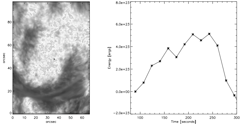
Figure 10. Microflaring event in the \text{Ly}\alpha plage. Left: The symbol 'x' marks the location of the brightening. Right: The energy estimate for this event.
