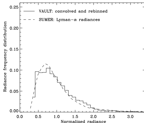
Figure 3. Normalized H I Ly \alpha distributions as obtained from SUMER data (dashed line) and the VAULT data (solid line) rebinned and convolved to match the SUMER spatial resolution after subtracting a background signal level of 80 \text{ DN s}^{-1} (see section 2.2).
