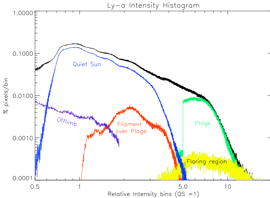
Figure 6. Ly \alpha emission histogram (black line). Different colors represent partial histograms from the labeled subregions. In particular we note that the "Quiet Sun" emissions spans one order of magnitude. Intensities are scaled to the median Quiet Sun level. Plot ordinates scaled to total number of data pixels. Cover area for each type (integral over the histogram curve) is: Total (black line): 100%, Quiet Sun: 61%, Plage:13%, Filament: 2%, Flaring region: 1%, Offlimb: 1%, Rest: 23%. See text on Section 8 for more details.
