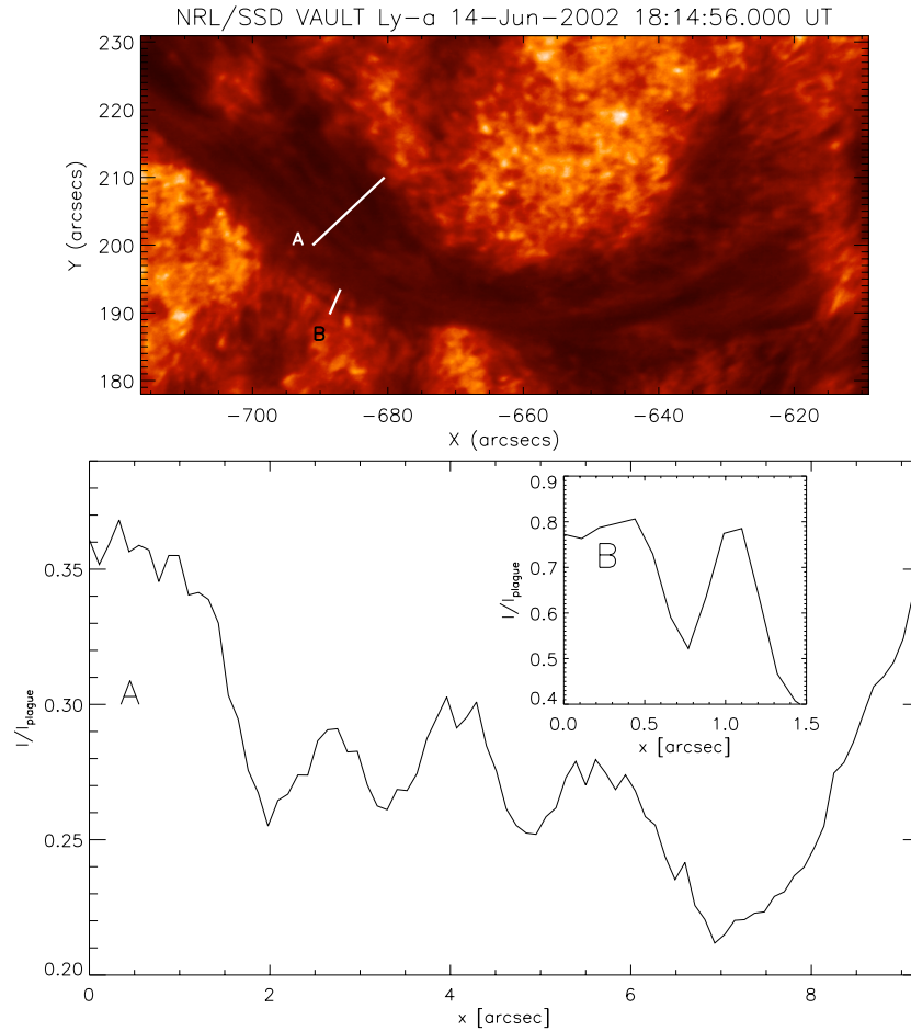
Figure 7. Prominence shows reduced absorption threads along its axis below 0.5'' . This supports a non-axisymmetric prominence. Top: Single VAULT frame, with labeled segments for the perpendicular cuts (labeled as 'A' and 'B'). Intensities are not scaled. Bottom: Intensity profile perpendicular to the prominence axis for 'A' segment and 'B' detached thread (plot inset). Intensities are scaled to surrounding median plage value.
