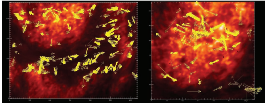
Figure 11. Detection of proper motions in Ly \alpha plage. The lengths of the displacement vectors are proportional to the estimated speed. Only pixels with correlation coefficients \geq 0.3 and intensity changes \geq 3\sigma above the background are considered. The units are VAULT pixels ( 0.112''/\text{pixel} ). Left: Filament and nearby plage. Upward motions can be seen along the western footpoint. Right: Plage detail. Note the counterstreaming motions along the filament boundary and diverging (explosive?) motions at certain bright points.
