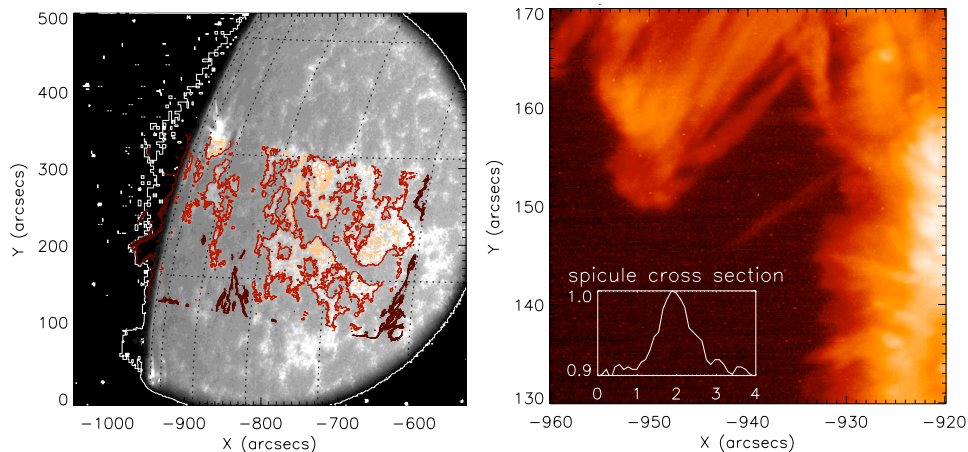
Figure 2. Left: Alignment of VAULT-TRACE \text{Ly}\alpha images. We find the best correlation by optimizing the position, rotation and scale in both x-y directions. We derive a pixel size of 0.125'' \times 0.110'' . The TRACE \text{Ly}\alpha was taken at 18:18:54 UT (B&W figure and white contour), the VAULT was taken at 18:17:30 UT (three red contours). Right: Estimation of the VAULT resolution using the thin spicule located at the center of the image. The median normalized cross section (in arcseconds) of the spicule along its length (plot inset in figure) is fitted with a gaussian, which leads to a FWHM \approx 0.49'' as an upper limit.
