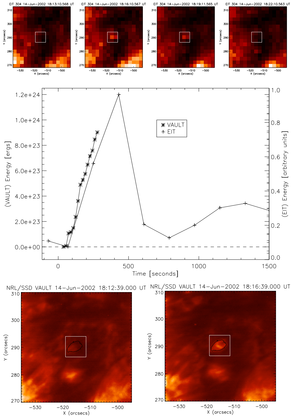
Figure 9. Microflaring event in the Quiet Sun detected in Ly\alpha and He II. Top panels: EIT He II images of the event. Middle panel: Comparison of the energy curves from VAULT to the EIT light curve. The total counts within the black outline (VAULT) and within the white boxes (EIT) were used to calculate the curves. Bottom panels: Ly\alpha images of the event at its initiation (left) and peak (right).
