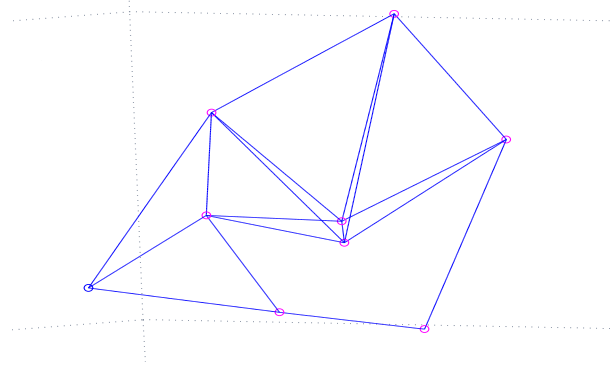
Figure 2: The Visibility Graph Based on the Interceptor's Initial Position and the Polygon Vertices for the Target Interception Example in Fig. 1.
