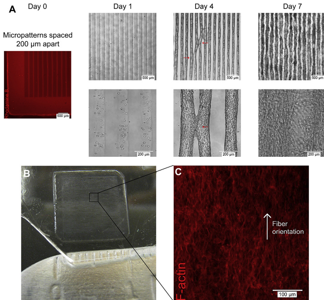
Fig. 7. Self-assembly of multiple aligned microconstructs into a macroscale and aligned 3D tissue construct. 3T3-fibroblast-laden 5% GelMA hydrogels patterned into rectangular microconstructs ( 50\ \mu\text{m} (w) \times 800\ \mu\text{m} (l) \times 150\ \mu\text{m} (h)) spaced 200\ \mu\text{m} apart self-assembled into macroscale and aligned 3D tissue constructs after 7 days of culture through convergence of multiple, aligned microconstructs. (A) Rhodamine B stained hydrogel shows initial microconstruct spacing of 200\ \mu\text{m} at day 0; representative phase contrast images of cell-laden microconstructs at day 1, 4 and 7 respectively show focal points of contact between neighboring aligned microconstructs at day 4 (red arrows) and convergence into a macroscale 3D tissue construct at day 7. (B) Image of a 1\ \text{cm} \times 1\ \text{cm} , self-assembled 3D tissue construct at day 7. (C) Representative F-Actin staining of middle xy-plane of macroscale 3D tissue construct shows orientated actin fiber organization in single direction.
