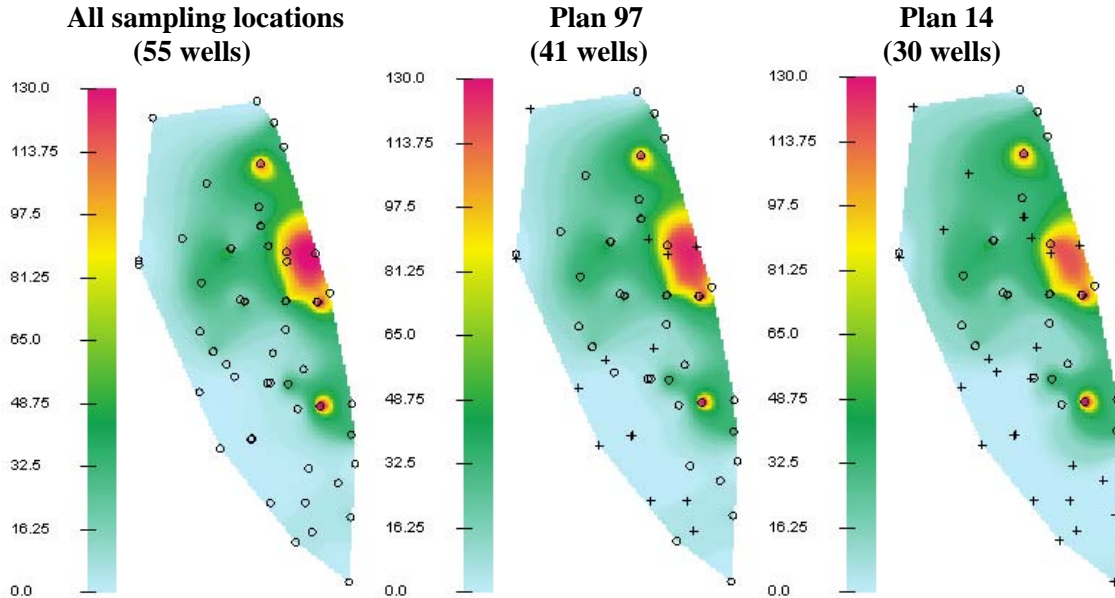
Figure 5-2. Example of Plume Maps for Plans Selected from Tradeoff Curve
