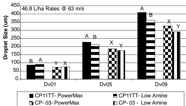
Figure 8. Droplet sizes for PowerMax and Low Mole Amine solutions at 46.8-L/ha spray rate in a 63-m/s airstream. (Within each droplet size category and nozzle type, means with the same letter are not significantly different.)
