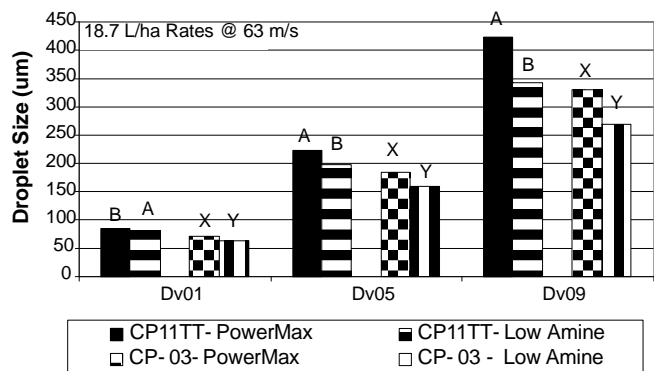
Figure 7. Droplet sizes for PowerMax and Low Mole Amine solutions at 18.7-L/ha spray rate in a 63-m/s airstream. (Within each droplet size category and nozzle type, means with the same letter are not significantly different.)
