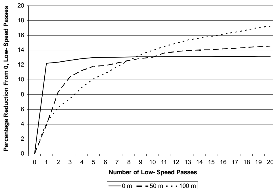
Figure 10. Percentage reduction in deposition at 0-, 50-, and 100-m downwind by number of spray passes made at 54 m/s as compared to all 20 spray passes made at 63 m/s (i.e. no 54-m/s passes).
