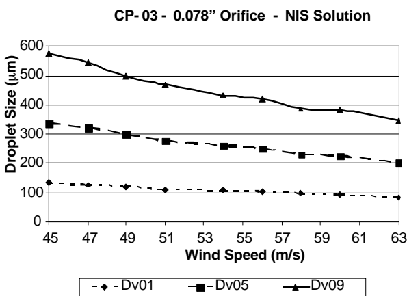
Figure 3. Effects of increasing airspeed on droplet size for the nonionic surfactant (NIS) solution.
