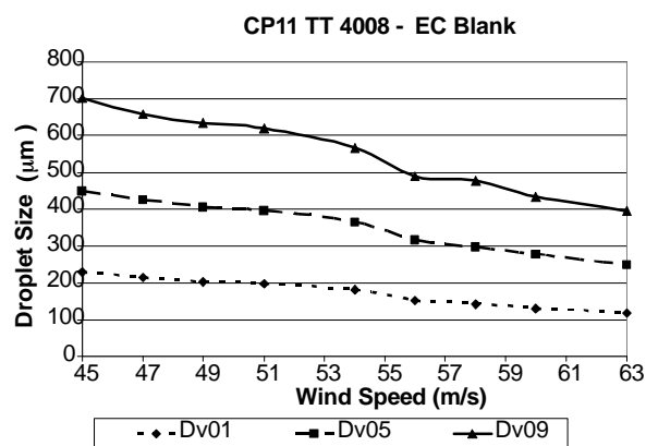
Figure 2. Effects of increasing airspeed on droplet size for the EC blank solution.
