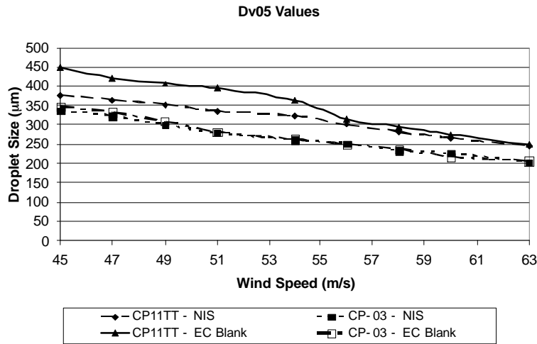
Figure 4. Comparison between measured DV0.5 values for the NIS and EC Blank solutions via different airspeeds with two nozzles.
