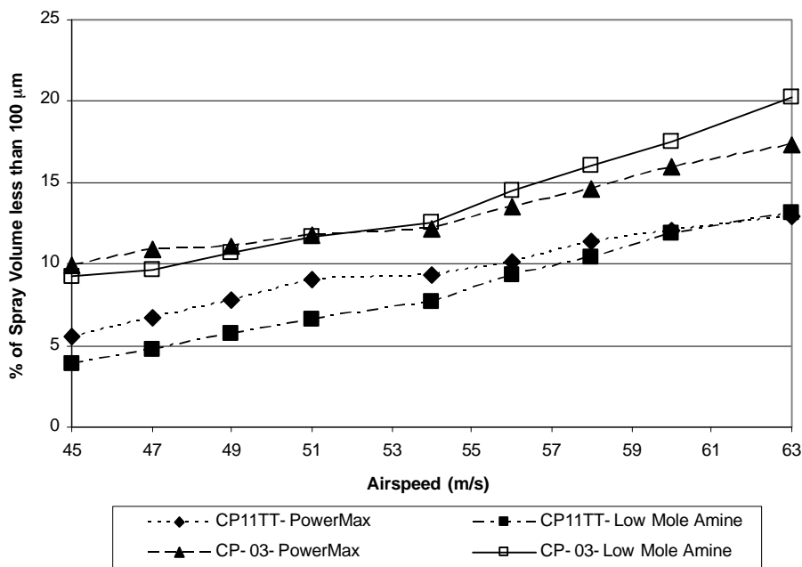
Figure 9. Percent of spray volume contained in droplets less than 100 µm for PowerMax and Low Mole Amine solutions in 45- to 63-m/s airstreams.
