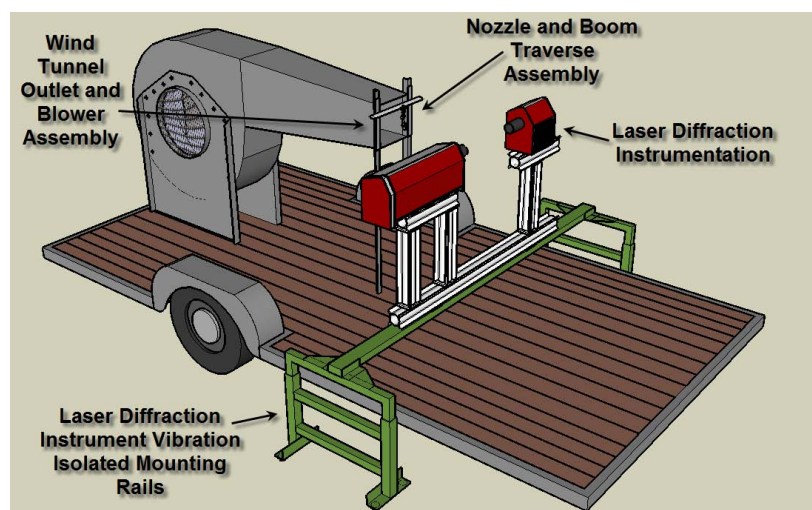
Figure 1. USDA-ARS high-speed wind tunnel.
