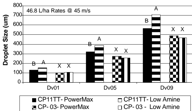
Figure 6. Droplet Sizes for PowerMax and Low Mole Amine solutions at 46.8-L/ha spray rate in a 45-m/s airstream. (Within each droplet size category and nozzle type, means with the same letter are not significantly different.)
