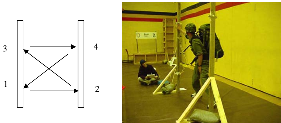
Figure 3: Wall Touch Test Setup
