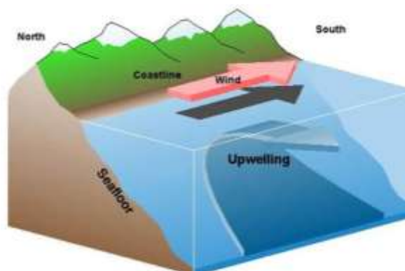
Figure 2-1: Schematic of Coastal Upwelling. ( http://www.greenseaupwelling.com/_images/upwellPic.png )
