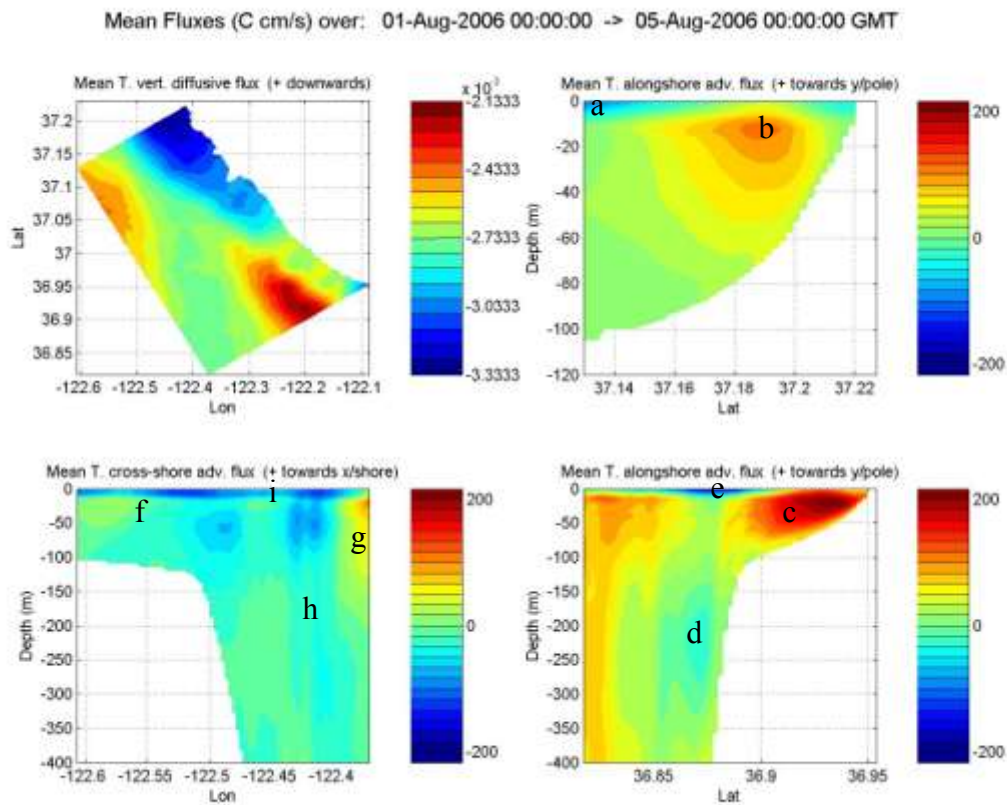
Figure 4-12: Heat Flux (C cm/s) through the Surface, North, South, and West Sections starting in Upper Left and going Clockwise for Run 11.
