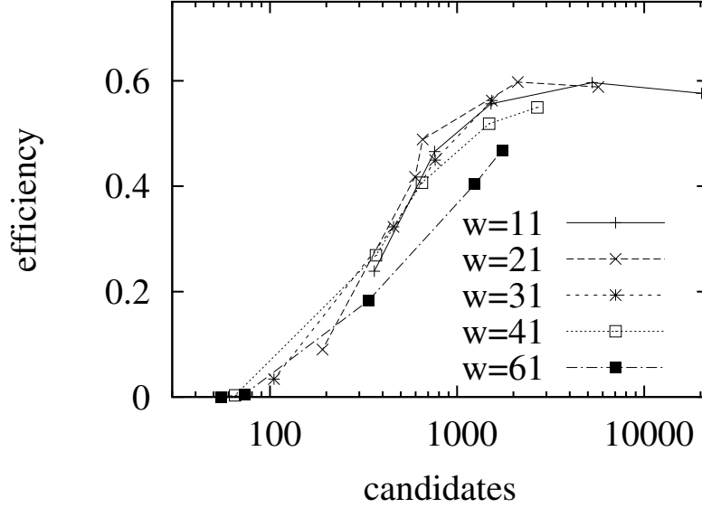
Figure 2.9: Efficiency plotted against the number of unidentified candidates (mostly false positives). Each line represents a different window size w , and each point represents the value of the efficiency at threshold \theta = 0.08, 0.10, 0.15, 0.20, 0.30 , the number of false positives monotonically grows with decreasing \theta (larger values of \theta on the left). All lines (all w values) show a plateau at different thresholds.
