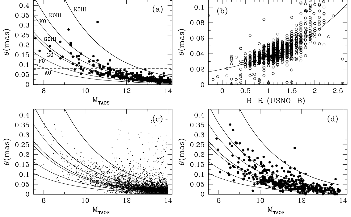
Figure 3.6: Angular size distribution for a typical TAOS field (field 120, RA: 13^\circ.7 , Dec: -10^\circ.7 ) derived from the 2MASS K - J colors (a). The curves show the theoretical behavior of the angular size for A0, F0, G0, K0 dwarf stars (thin lines) and G0, K0, K5 giants (thick lines). The size of the Fresnel scale at 43 AU is shown at 0.08 mas (dashed line). Best fit to the angular size distribution (b): x -axis is the USNO-B B - R color and y is the angular size derived using Equations 3.2 & 3.3, converting all stars to apparent magnitude R = 12 . Implanted angular sizes, derived from USNO-B the B - R color for our simulation (c) and angular size of the star for which events are recovered (d); a random subset of 1% of our data is plotted in the bottom panel.
