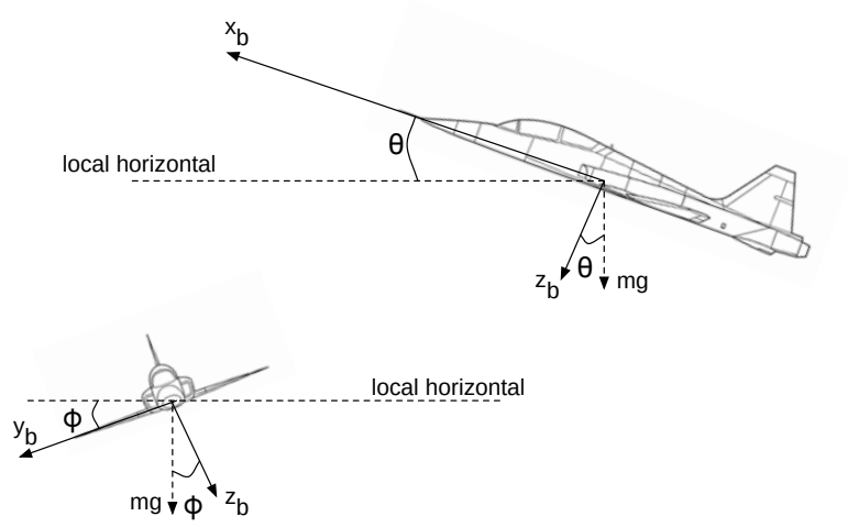
Figure 3.3: Gravity vector in relation to aircraft body coordinates.
