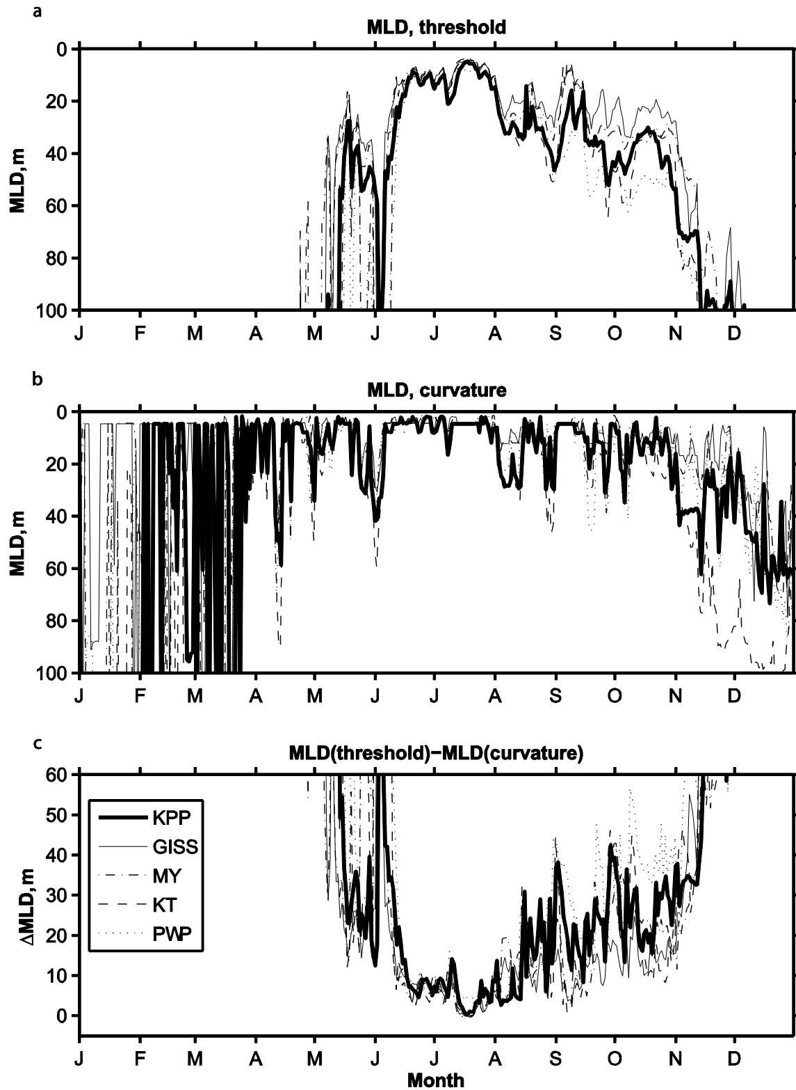
Figure 6. Times-series of (a) threshold MLD, (b) curvature MLD, and (c) threshold minus curvature MLD difference from a point in the gulf of Lyons (42.09°N, 5°E) The line-styles listed in the legend are the results from the five mixing models.
