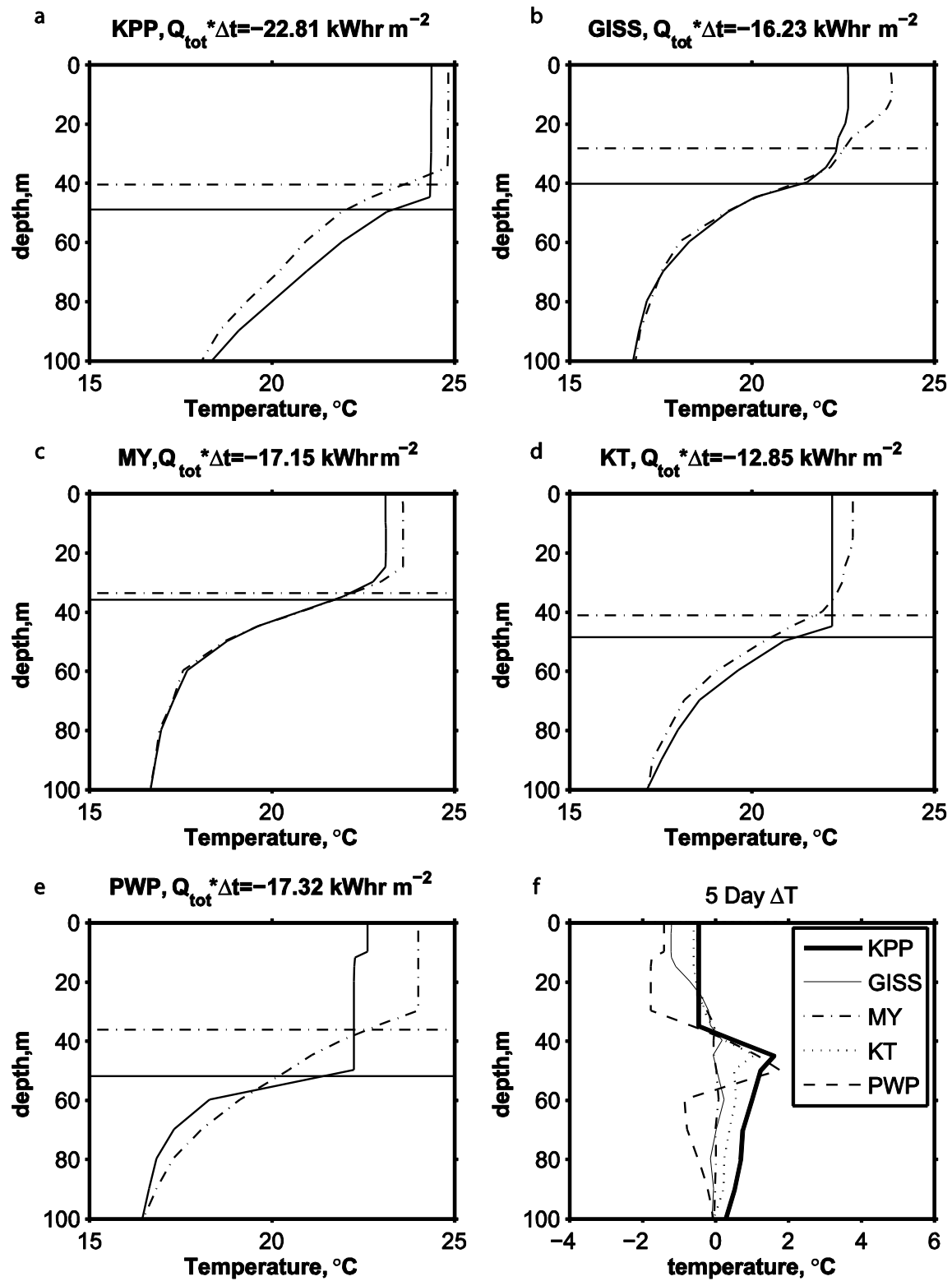
Figure 14. An example profile located in the Rhodes Gyre region in the same location as in Figure 12. Each panel is also in the same format as in Figure 13 except that the five day interval starts on October 16 th and ends on October 20 th 2006 and is during a surface cooling period.
