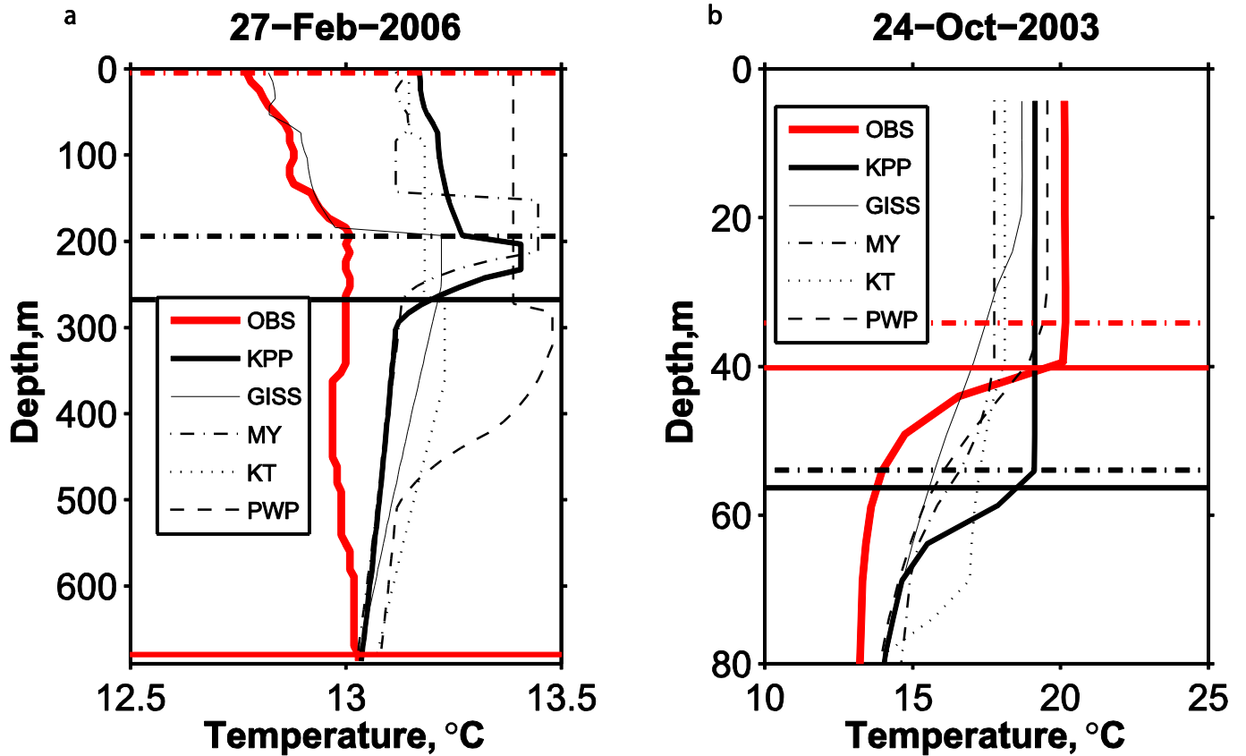
Figure 17. Example observation profiles (red curves) from the Gulf of Lyons region on (a) 27 February 2006 and (b) 24 October 2003. The black curves are model results for the same time and location as the observation for the five mixing model case shown in the legend, which identifies the line-style. The red horizontal lines are the threshold MLD (solid red) and the curvature MLD (red dashed-dot) from the observation profile. The black horizontal lines are the threshold MLD (solid black) and the curvature MLD (black dashed-dot) from the KPP mixing model case.
