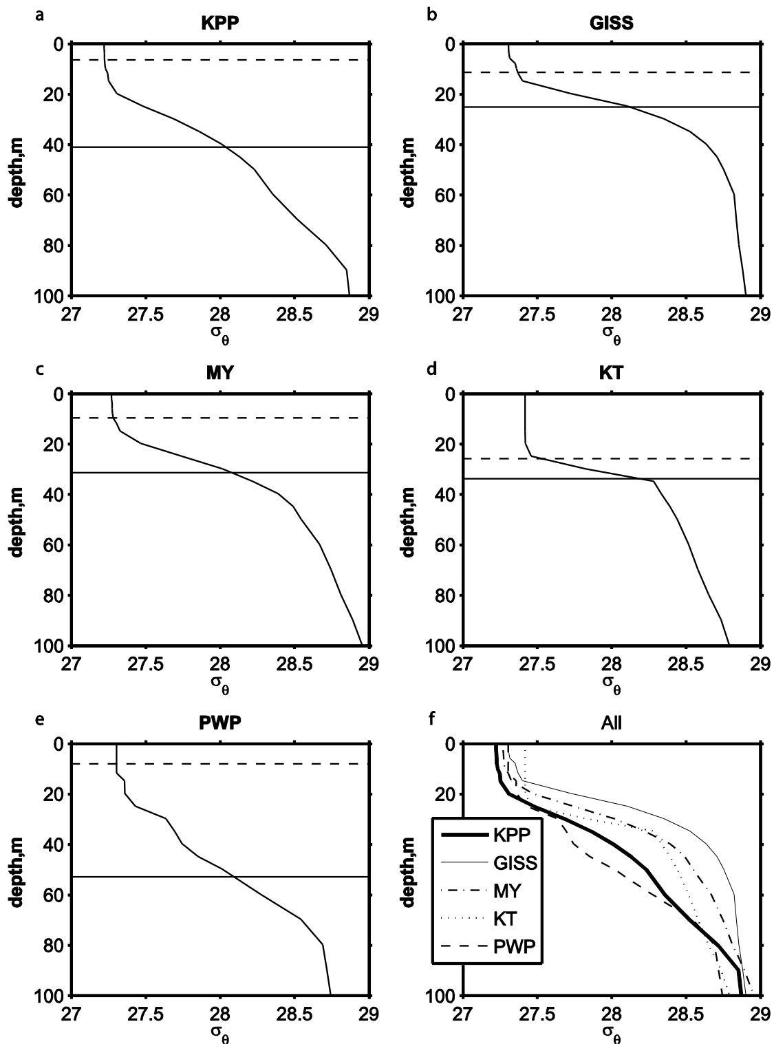
Figure 8. An example summer profile from Gulf of Lyons (42.09°N, 5°E) during 27 October 2006 from the (a) KPP, (b) GISS, (c) MY, (d) KT, and (e) PWP mixing model runs. Plot (f) shows profiles from all mixing models for comparison. The solid (dashed) lines in (a) through (e) represent the threshold (curvature) MLD.
