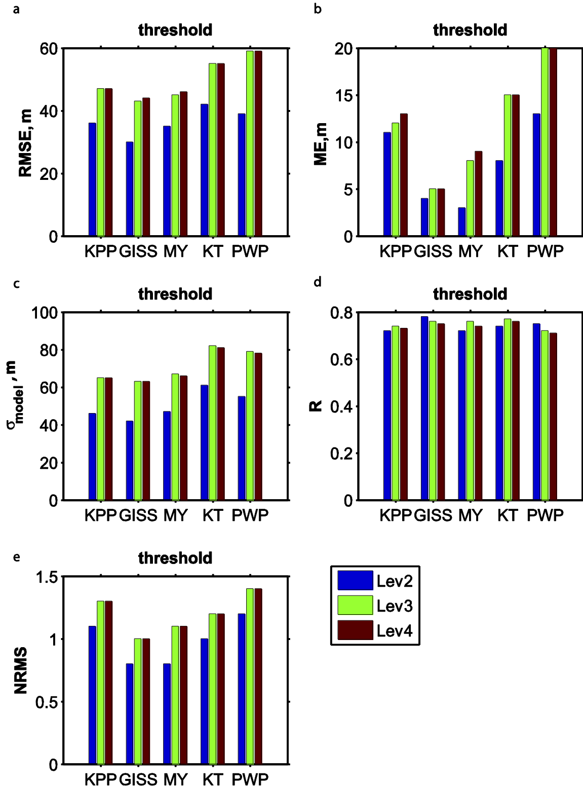
Figure 15. Validation result using the threshold MLD definition for (a) RMSE, (b) ME, (c) model standard deviation ( \sigma_{model} ), (d) R, (e) NRMS and each mixing model indicated at the bottom of each plot. The bar graph colors represent data editing levels 2, 3, and 4 as indicated in the legend.
