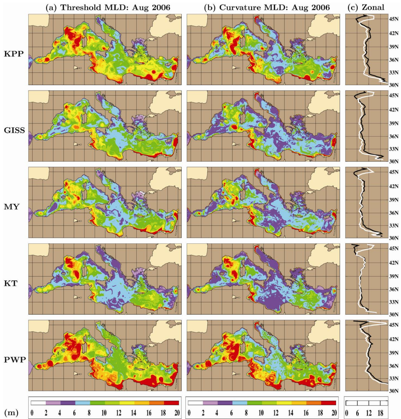
Figure 4. The same as Figure 3 but in August 2006. Note that the color palette range is different to better demonstrate spatial variability of summer MLD.
