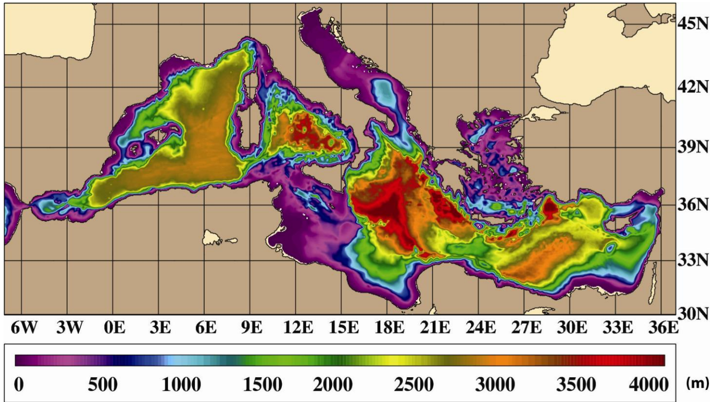
Figure 1. Bottom depth (m) in the Mediterranean Sea as constructed from the 1 minute resolution General Bathymetric Chart of the Oceans (GEBCO) which is available online at http://www.gebco.net/ . There are large regions where the depths are shallow (e.g., < 500 m), such as most of the Adriatic and Aegean Seas. The land-sea boundary (in light tan) is set at 5 m, i.e., water depths < 5 m are excluded and considered as land for the ocean model simulations. We use this domain and drop the latitude and longitude labels from rest of the similar figures for simplicity.
