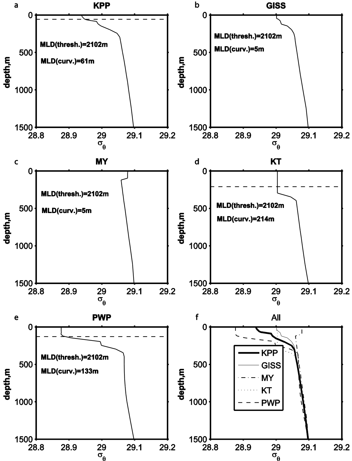
Figure 7. An example winter profile from Gulf of Lyons (42.09°N, 5°E) during February 20 th 2006 from the (a) KPP, (b) GISS, (c) MY, (d) KT, and (e) PWP mixing model runs. Plot (f) shows profiles from all mixing models for comparison. The dashed lines in (a) through (e) represent the curvature MLD while the threshold MLD is at the bottom of the profile as indicated inside each plot.
