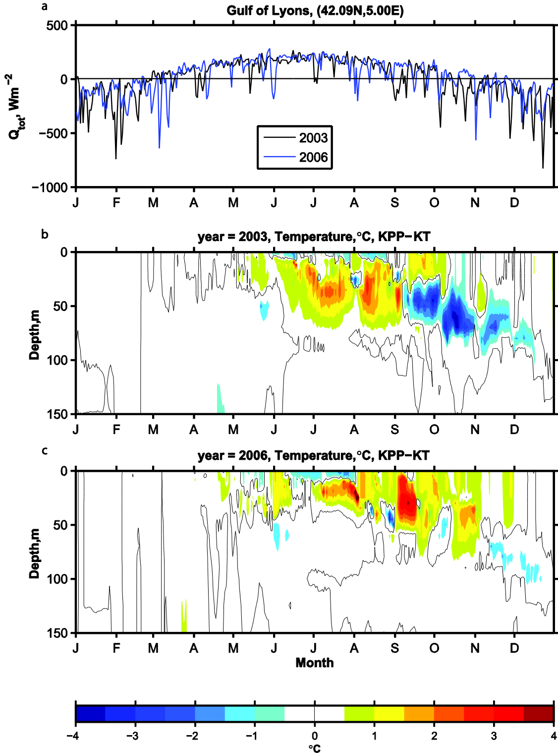
Figure 9. One year time series for a point in the Gulf of Lyons located at 42.09°N, 5°E for 2003 and 2006 of (a) total surface flux ( Q_{tot} ) positive into the ocean in W m^{-2} and subsurface temperature differences for KPP-KT versus depth in °C for (b) 2003 and (c) 2006. In (a) the black line is Q_{tot} for 2003 and the blue line is Q_{tot} for 2006.
