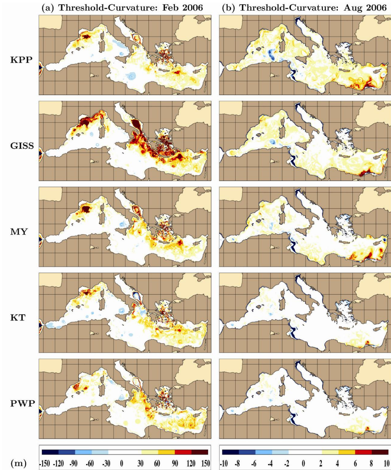
Figure 5. Spatial variability of threshold minus curvature MLD differences for (a) February and (b) August 2006.
