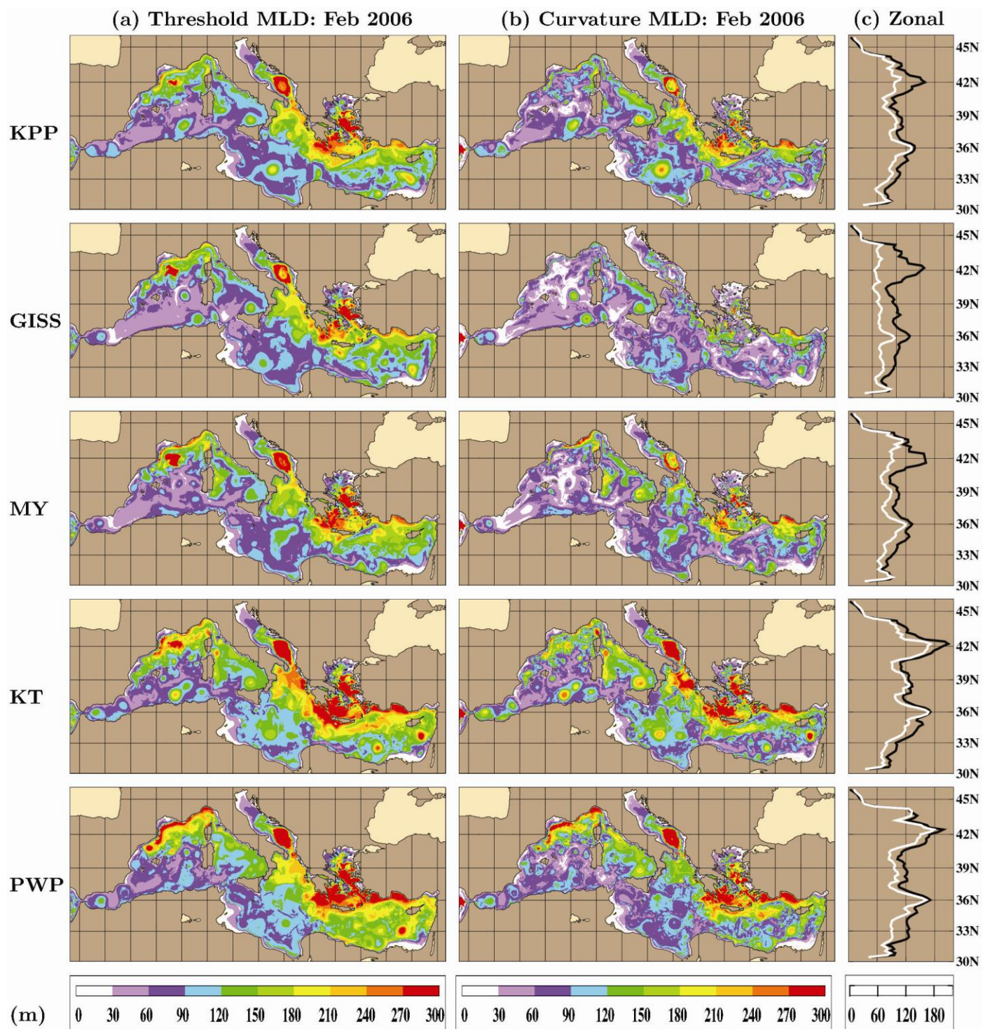
Figure 3. Spatial variations of mean MLD predicted by five mixing models in February 2006. MLD is computed based on two methodologies as described in the text: the (a) threshold and (b) curvature MLD definition. Also included in (c) are the zonal averages of MLD (the threshold MLD in black and the curvature MLD in white).
