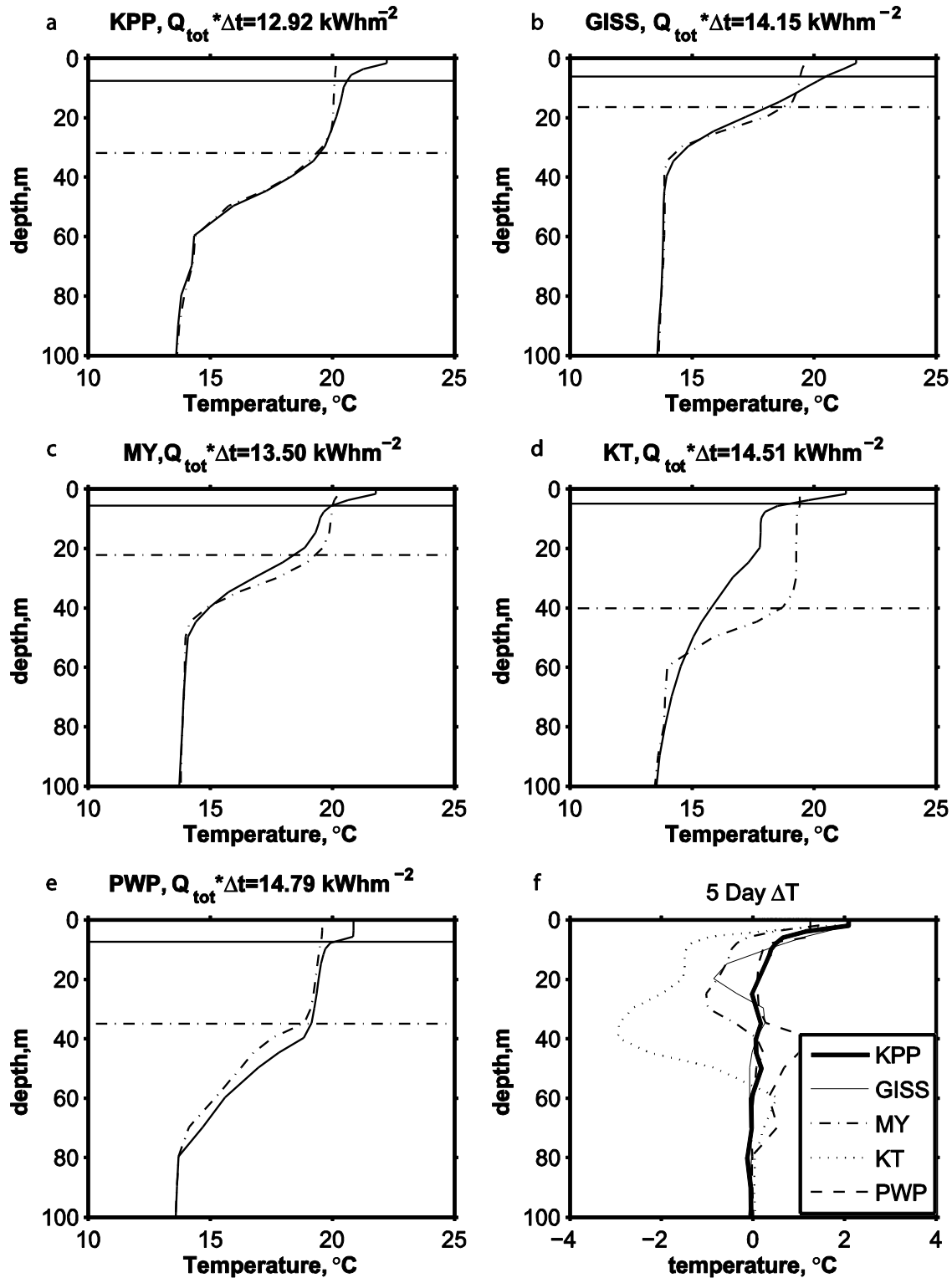
Figure 11. An example profile located in the Gulf of Lyons in the same location as in Figure 10. Each panel is also in the same format as in Figure 10 except that the five day interval starts on September 1 st and ends on September 5 th 2006 and is during a warming period.
