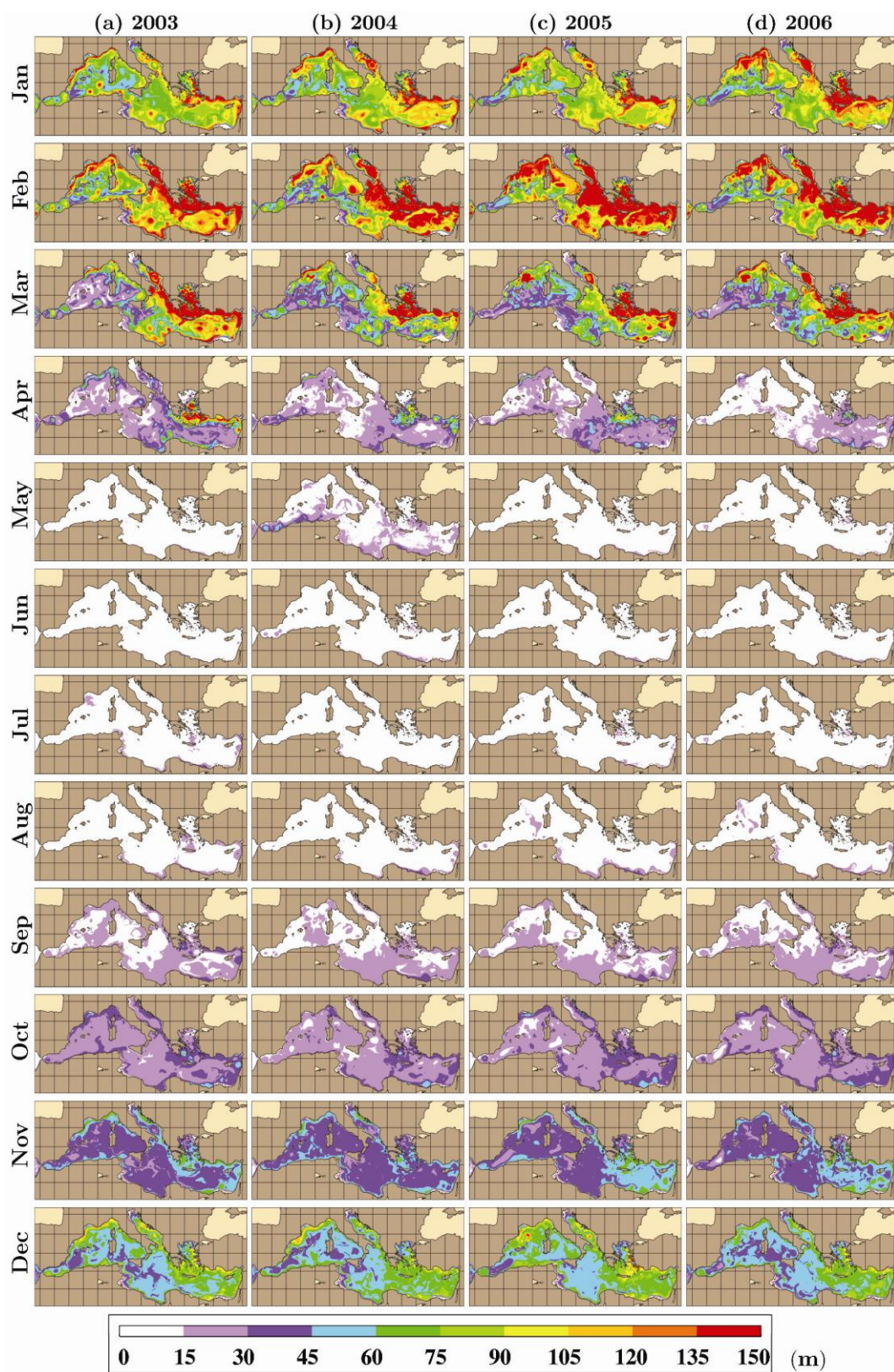
Figure 2. Monthly mean threshold MLD fields in the Mediterranean Sea from 2003 through 2006 from the MY mixing model simulation.
