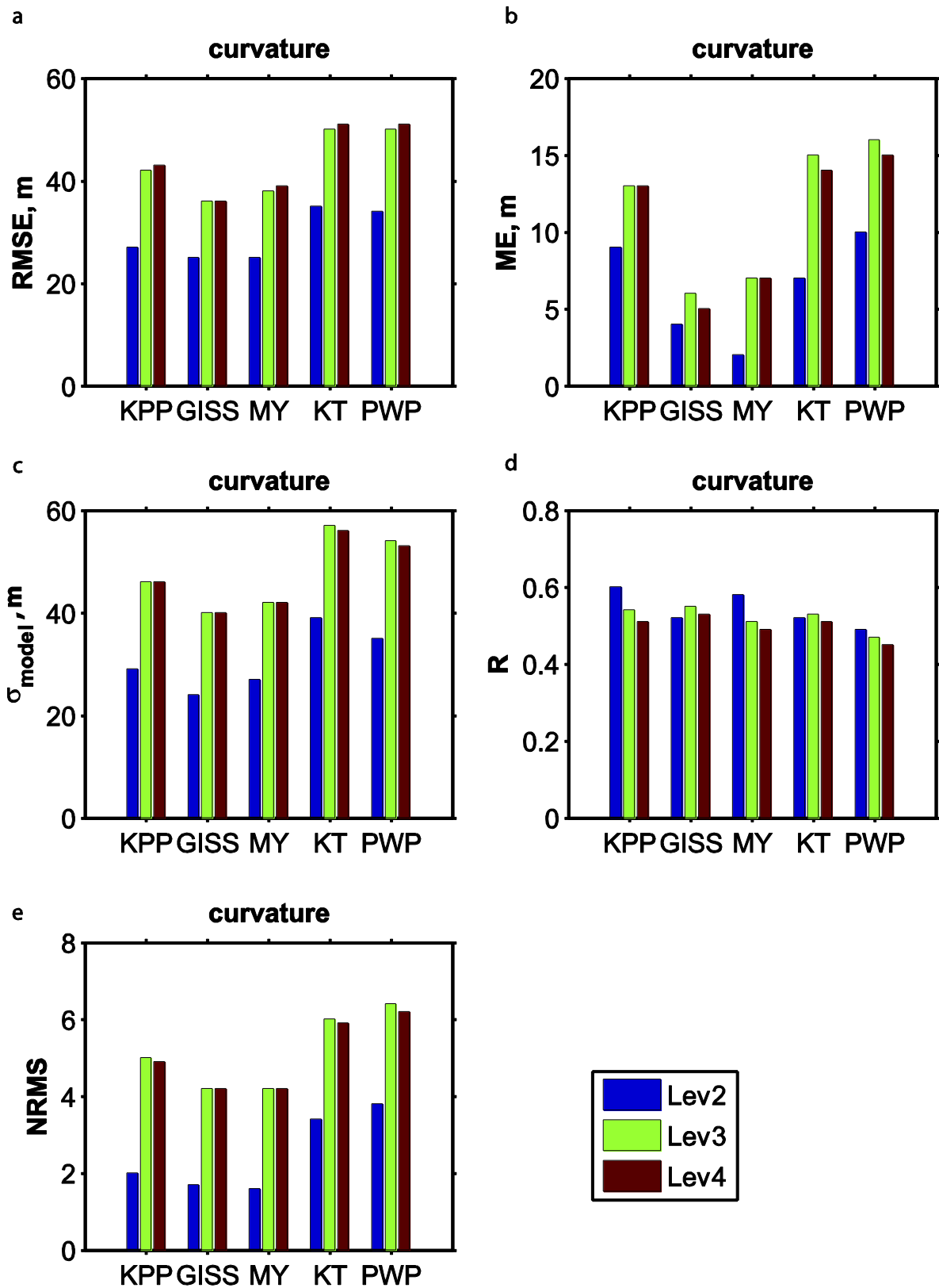
Figure 16. Validation result using the curvature MLD definition for (a) RMSE, (b) ME, (c) model standard deviation ( \sigma_{\text{model}} ), (d) R, (e) NRMS and each mixing model indicated at the bottom of each plot. The bar graph colors represent data editing levels 2, 3, and 4 as indicated in the legend.
