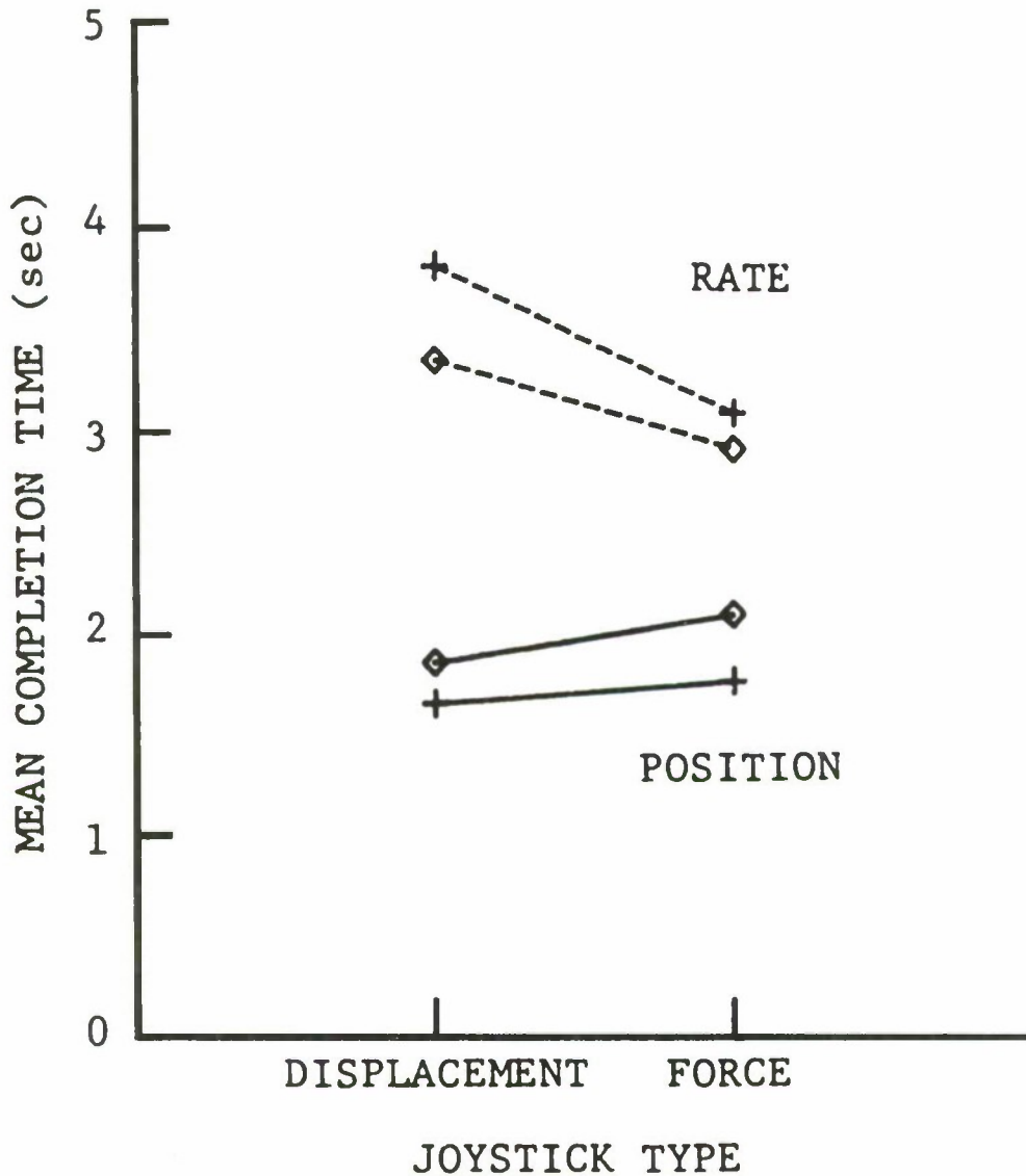
FIGURE 9 Displacement and force joystick control.
