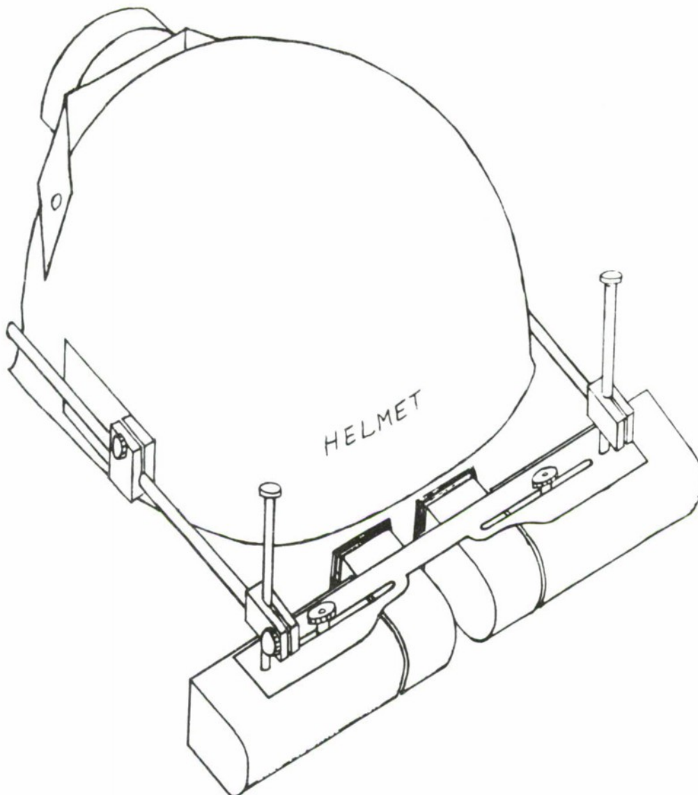
FIGURE 5 Current HMD design.
