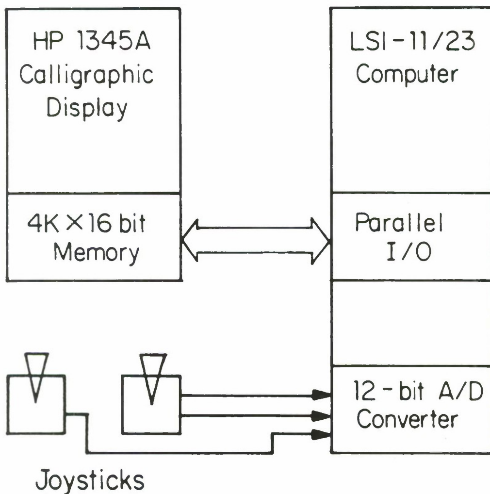
FIGURE 1 Experimental arrangement.
