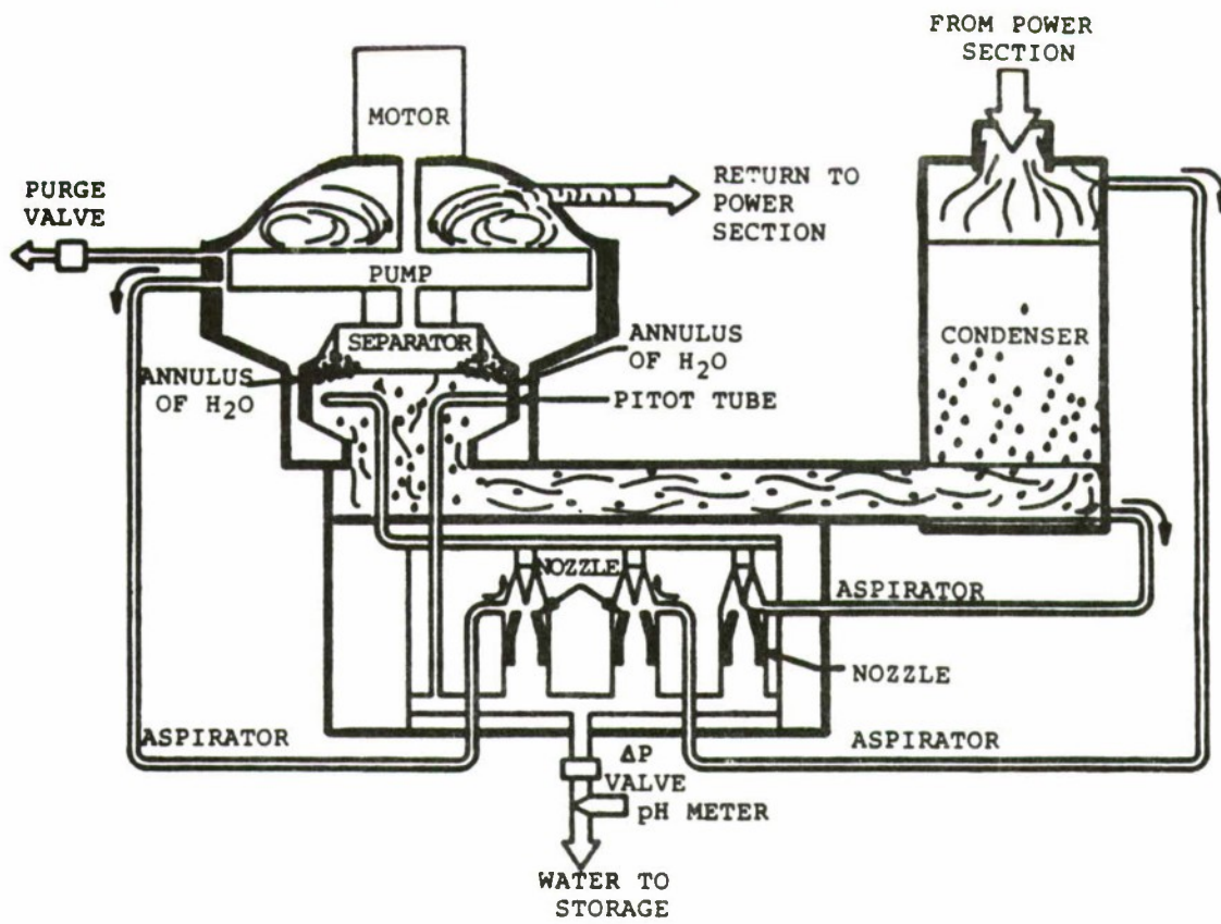
FIGURE 2 Details of the water separation unit. Source: Gerald Eichhoefer (July 1985).
