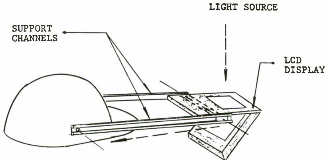
FIGURE 4: Early HMD design with LCD screen.
