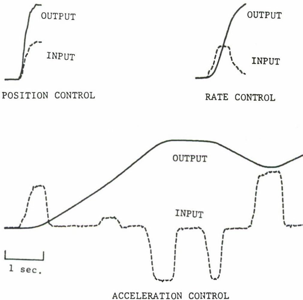
FIGURE 8 Position, rate and acceleration control.
