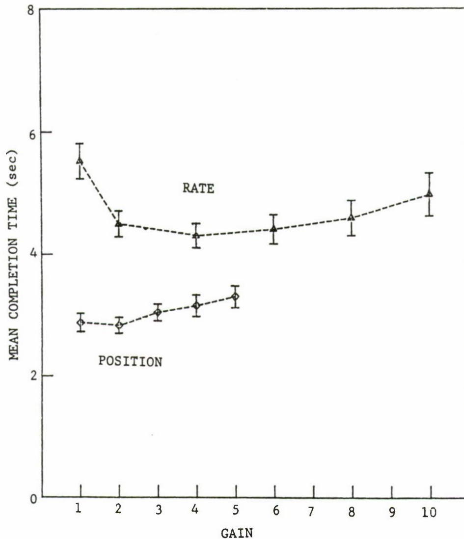
FIGURE 7 Performance comparison of position and rate control.
