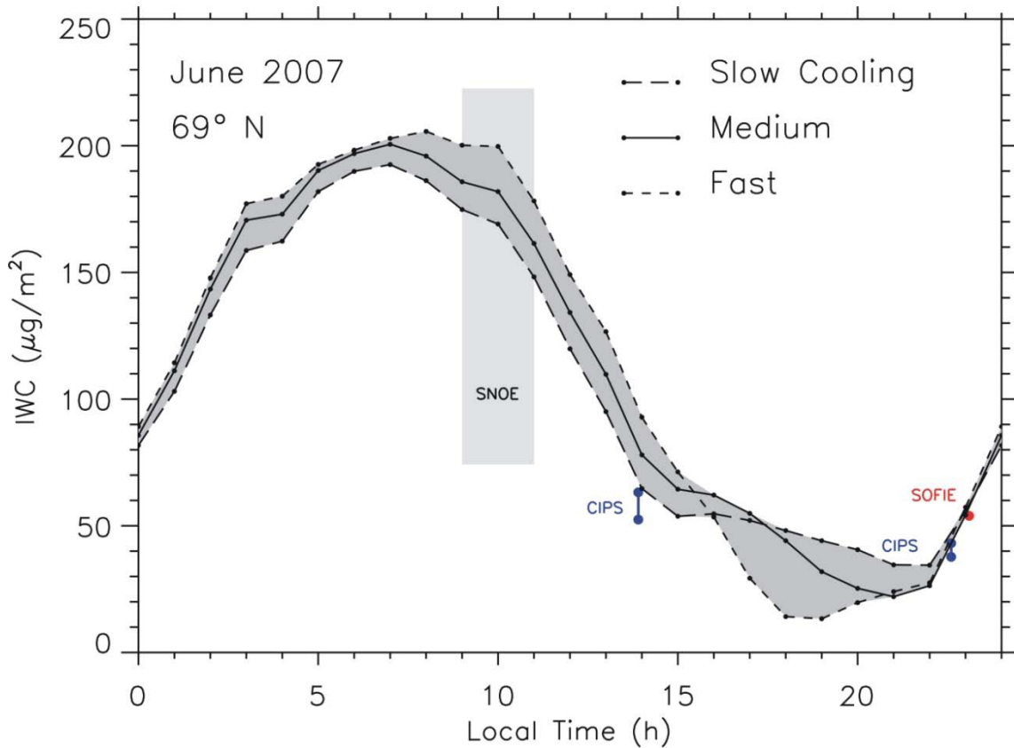
Figure 7. The calculated IWC over the diurnal cycle at 69^\circ N for June, 2007. Three different solutions are presented representing three assumed parcel cooling rates: Slow (0.50 K/hr), Medium (0.68 K/hr) and Fast (1.00 K/hr), where the shading represents the range within these solutions (see text). AIM/CIPS (blue) and AIM/SOFIE (red) data from the same time period are overplotted. The CIPS observations are averaged over a 3^\circ latitude band around 69^\circ N and have been scaled up to be consistent with simultaneous SOFIE observations in separate common volume observations. Also shown are observations from SNOE, which were collected between 0900-1100 LT and have been scaled upwards for representative solar minimum conditions.
