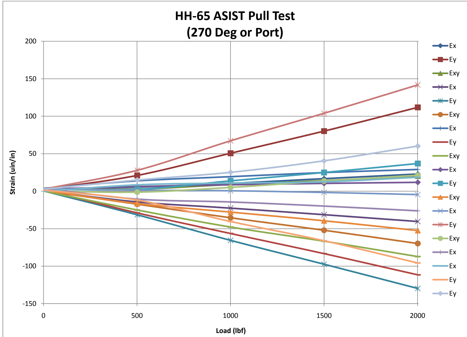
Figure B8 - Load Versus Strain Plot 270 deg. Load Case
