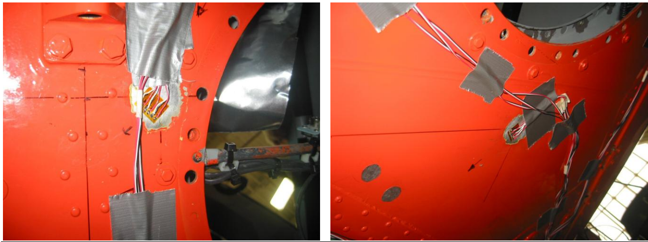
Figure 17 –Examples of Actual Locations for Gauges at Locations (a) and (e) on Belly of Aircraft
