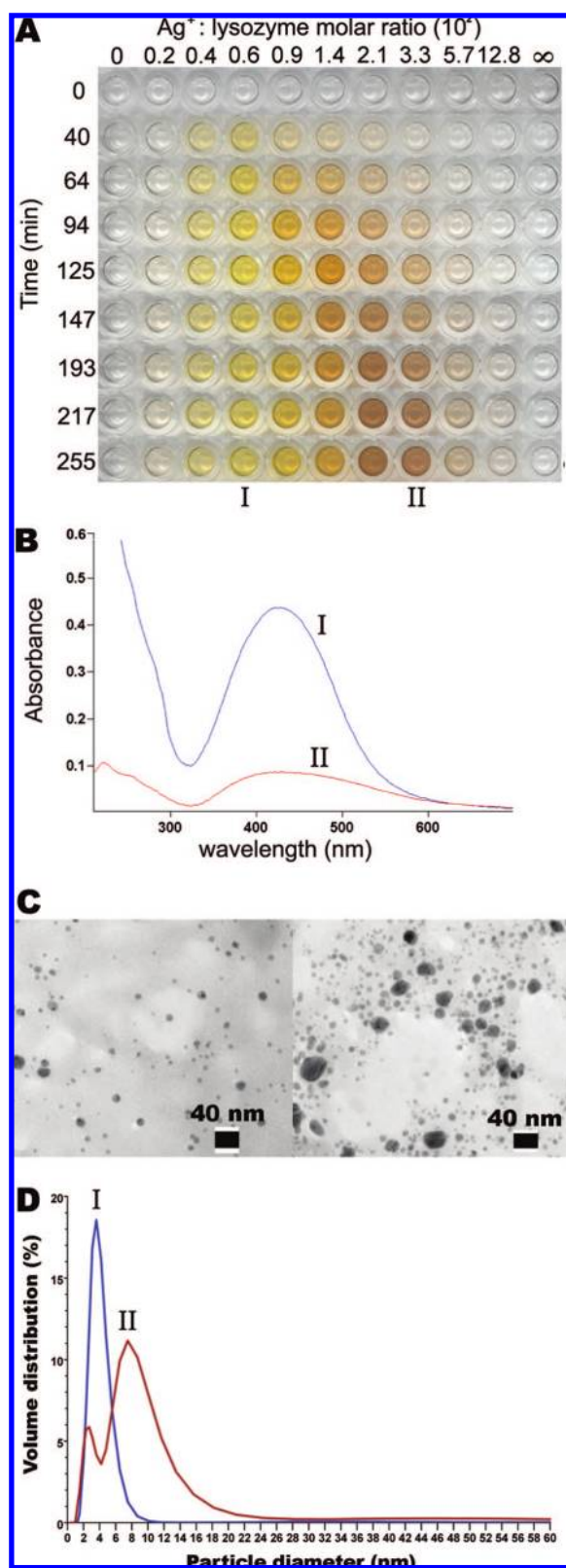
Figure 1. Lysozyme and silver acetate solutions were mixed in varying molar ratios and exposed to light over the course of 255 min. At set time intervals, reactions were added to a row of microtiter plate wells and imaged using a document scanner (A). Representative samples of yellow (I) and red (II) nanoparticles from the synthesis assay were used in absorbance spectroscopy (B), TEM imaging (C), and dynamic light scattering to determine nanoparticle size distribution (D).
