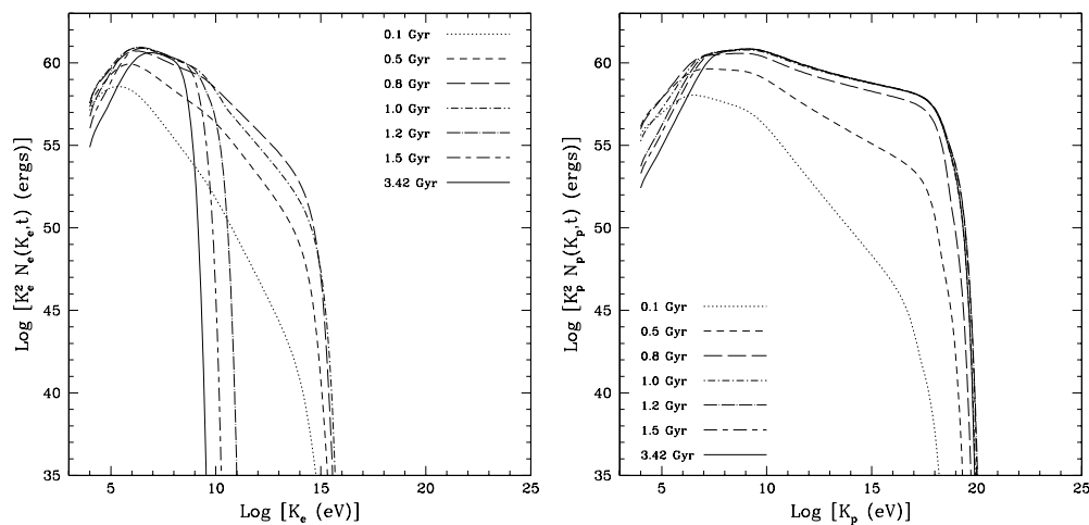
FIG. 4.—Primary electron ( left ) and proton ( right ) energy spectra for a shock formed by a merging cluster using a standard parameter set with M_1 = 10^{15} M_\odot , M_2 = 10^{14} M_\odot , and B = 1.0 \mu\text{G} . The interaction begins at redshift z_i = 0.3 and is evolved to the present time ( z = 0.0 ; solid curve ) with spectra shown at the various times given in the figure. The redshifts corresponding to the time delays of 0.1, 0.5, 0.8, 1.0, 1.2, 1.5, and 3.42 Gyr are z = 0.289, 0.248, 0.218, 0.199, 0.180, 0.153, and 0.0 , respectively. Particle injection ends at t_{\text{acc}} \cong 1.1 \text{ Gyr} (see discussion following eq. [19]).
