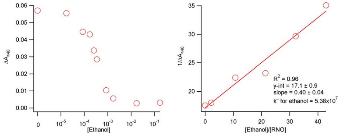
Figure 29: Typical competition kinetic plots. (A) Change in absorbance at 440 nm (indicating change in concentration of PNDA over 90 min); (B) Linear version of 1st six data points, used to calculate k'' .
