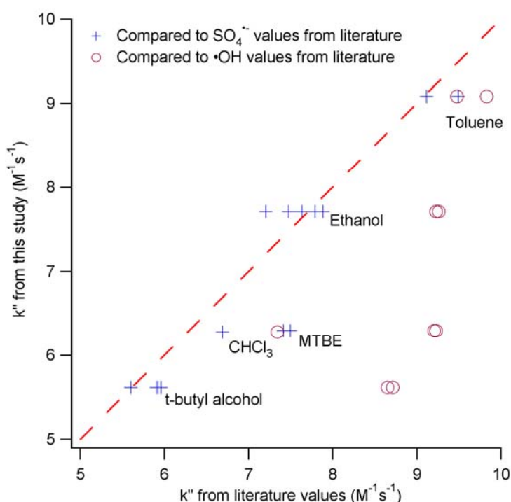
Figure 31: The values of k'' obtained by this study with competition kinetics compared with values of k'' for \bullet\text{OH} and \text{SO}_4^{\bullet-} obtained with either COC or \text{SO}_4^{\bullet-} in excess (literature values).
