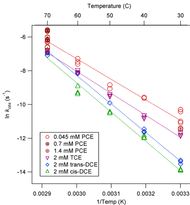
Figure 40 Arrhenius plots for the chlorinated ethenes. Experimental conditions: unbuffered, 10:1 molar ratio of \text{Na}_2\text{S}_2\text{O}_8 to chlorinated ethenes. Initial concentrations are given in the legend.
