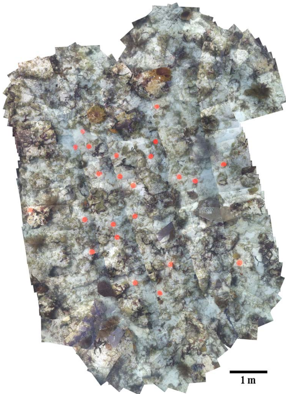
Fig. 3 Video mosaic constructed with video collected from a hand-held digital camcorder in June 2004 at Brooke's Reef in the Florida Reef Tract (depth 7–10 m). The video was collected
