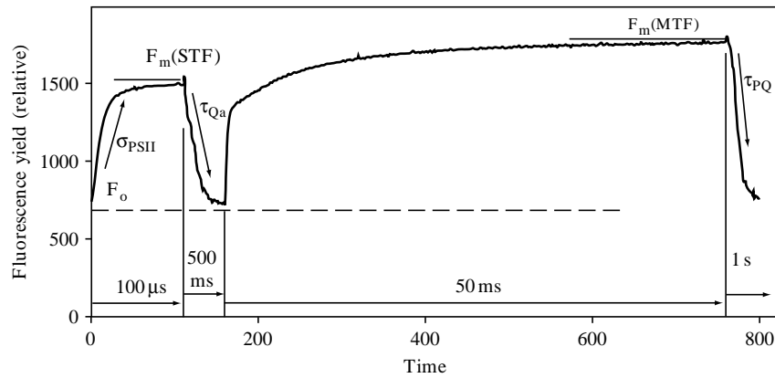
Figure 1: An example of the FIRE measurement protocol consisting of four phases: (1) a strong short pulse of 100 \mu\text{s} duration (called Single Turnover Flash, STF) is applied to cumulatively saturate PSII and measure the fluorescence induction from F_o to F_m(\text{STF}) ; (2) weak modulated light is applied to record the relaxation kinetics of fluorescence yield on the time scale of 500 ms; (3) a strong long pulse of 50 ms duration (called Multiple Turnover Flash, MTF) is applied to saturate PSII and the PQ pool; (4) weak modulated light is applied to record the kinetics of the PQ pool re-oxidation the time scale of 1 s. Analysis of the Phase 1 provides F_o , F_m , F_v/F_m(\text{STF}) , \sigma_{\text{PSII}} , p ; Phase 2 – time constants for the electron re-oxidation on the acceptor side of PSII (i.e., re-oxidation of the Q_a acceptor); Phase 3 – F_m(\text{MTF}) and F_v/F_m(\text{MTF}) ; Phase 4 – the time constant for the electron transport between PSII and PSI (re-oxidation of the PQ pool).
