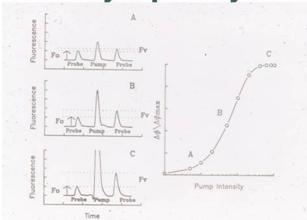
Pump-and-probe technique
