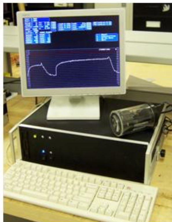
Developed FIRE System ( F luorescence I nduction and R elaxation)
