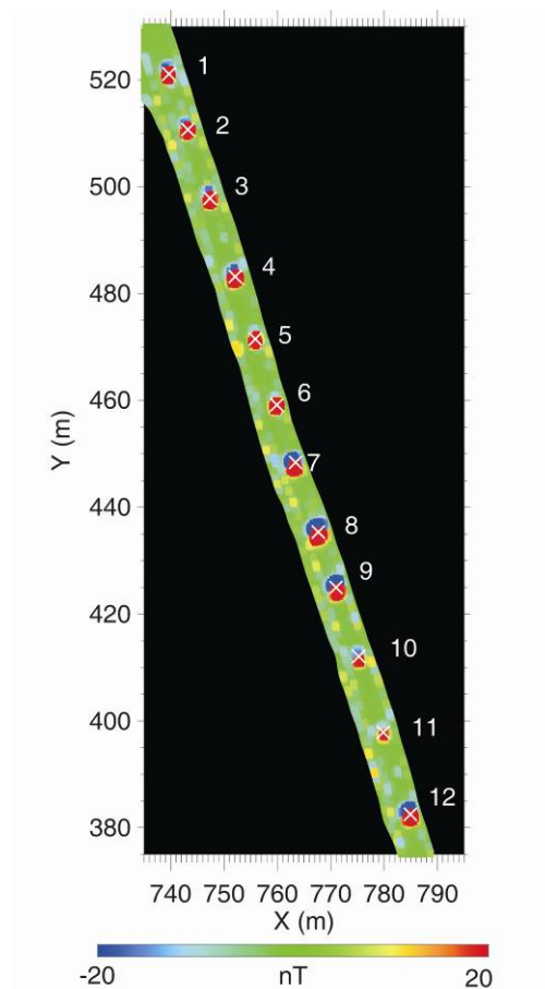
Figure 5-7. This is a magnetic anomaly image of the targets in the Calibration Line from a 3-pass survey made by the MTA.
