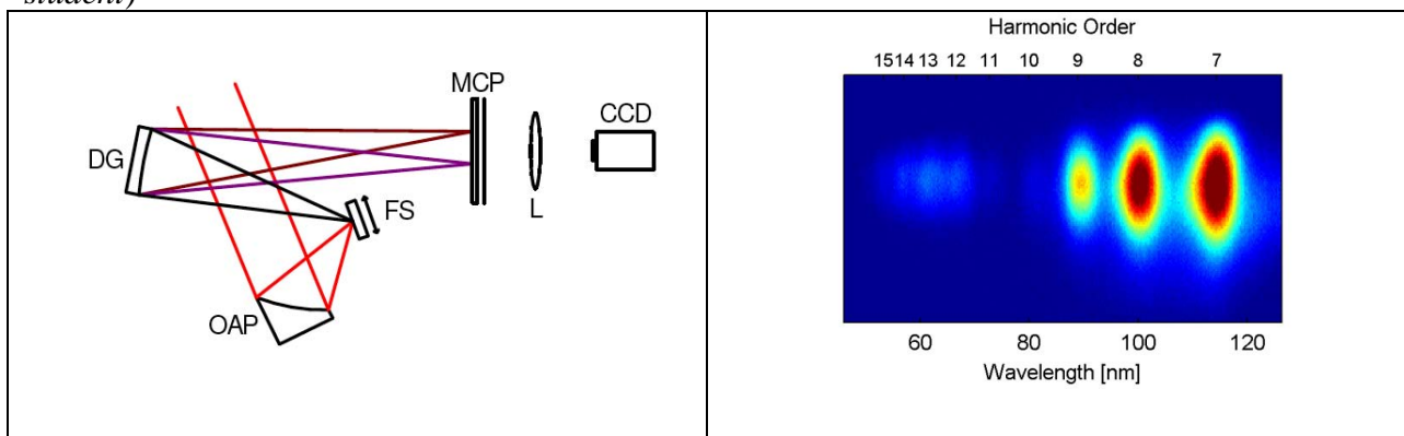
High-order harmonic generation experimental geometry.
