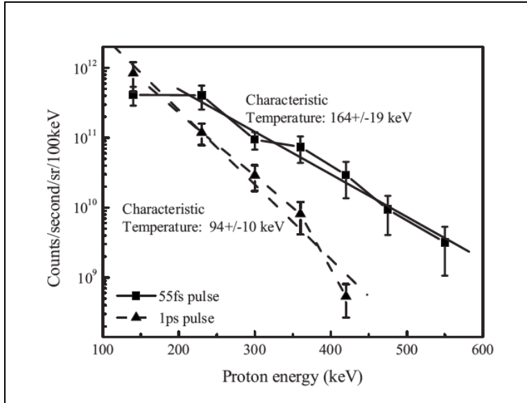
Proton spectra arising from irradiation of a glass target with 55fs and 1 ps pulses. Water and oil adhering to the target surface are the likely sources of protons driven by TeV/m electric fields.
