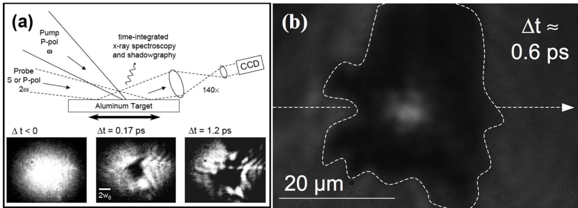
Fig. 1. Summary of measurements of surface heat transport for Al target excited at relativistic intensity. (a) Experimental setup for femtosecond microscopy with selected images from [2] of the heated plasma using p-polarized probe at the indicated time delays \Delta t and focused pump intensity I_{\text{pump}} \approx 1e18 \text{ W/cm}^2 (bottom). (b) New probe image as in (a), but for \Delta t = 0.6 \text{ ps} and I_{\text{pump}} \approx 3e18 \text{ W/cm}^2 . The bright central spot is second-harmonic radiation generated by the focused pump that was scattered into the probe imaging system. Reduced reflectivity region, outlined by dashed curve, is \sim 25 \mu\text{m} in diameter..
