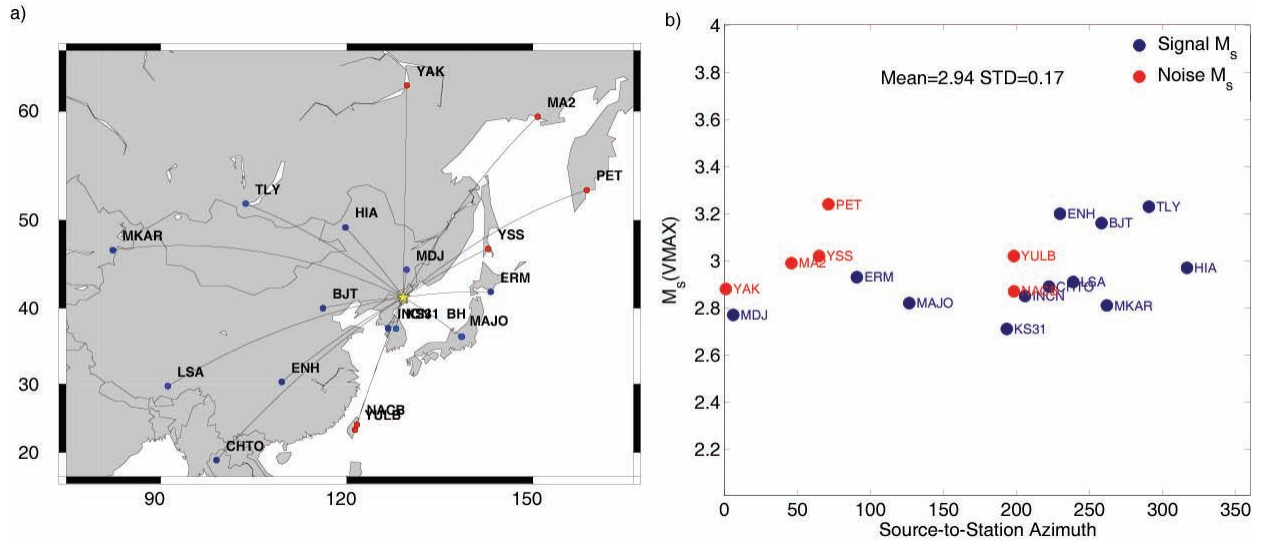
Figure 4. Signal- and noise-based M_s (VMAX) estimates for the 9 October 2006 North Korean event. a) Map of stations showing where noise-based (red circles) and signal-based (blue circles) surface wave magnitudes were estimated. b) Station magnitudes show a network average of 2.94, which considers only signal-based (blue) measurements.
